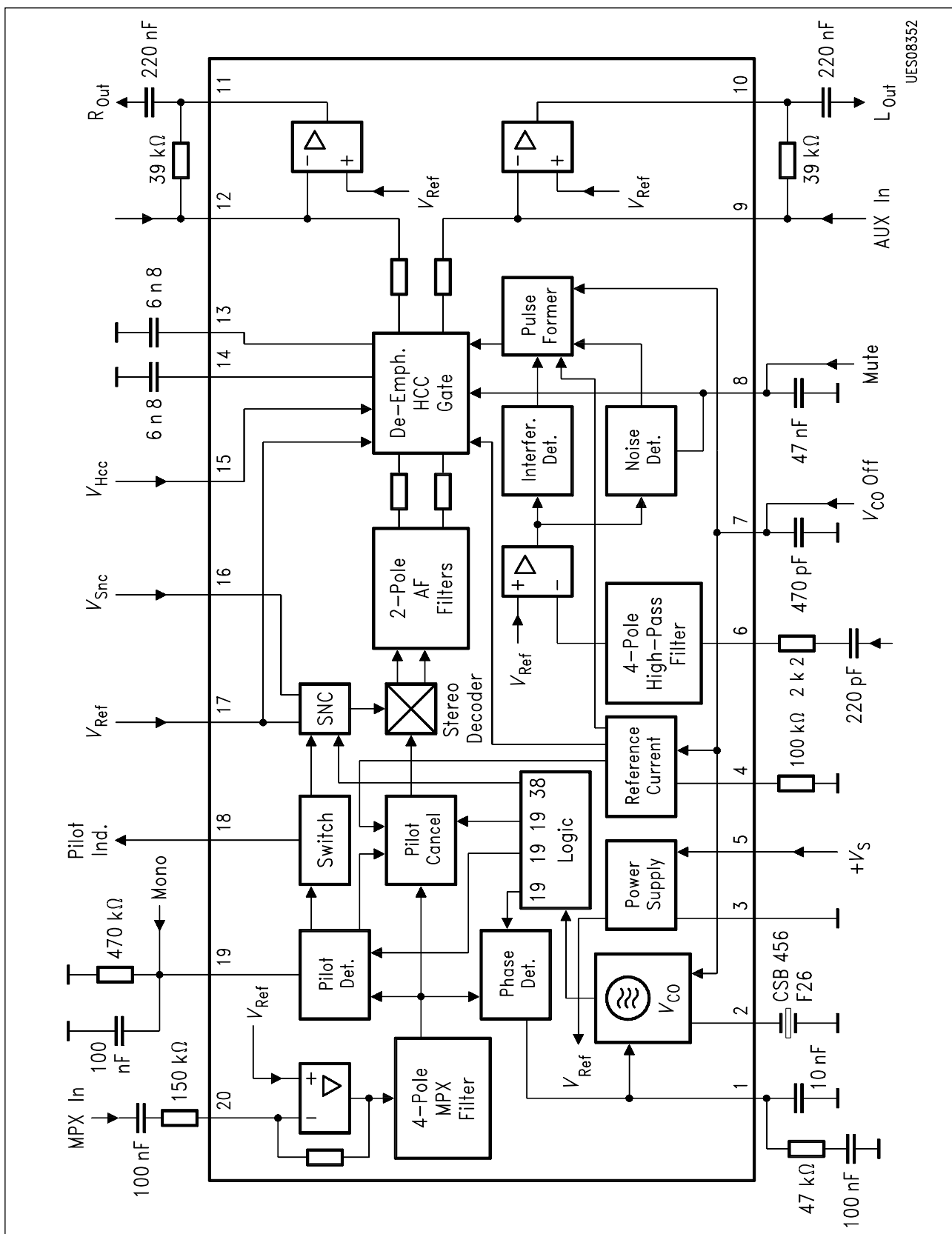
Figure 3 Test Circuit
