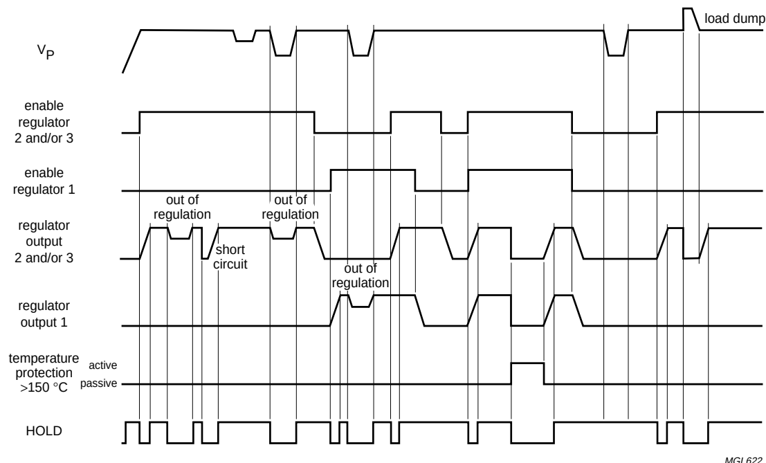
Fig.4 Timing diagrams of the HOLD signal.
