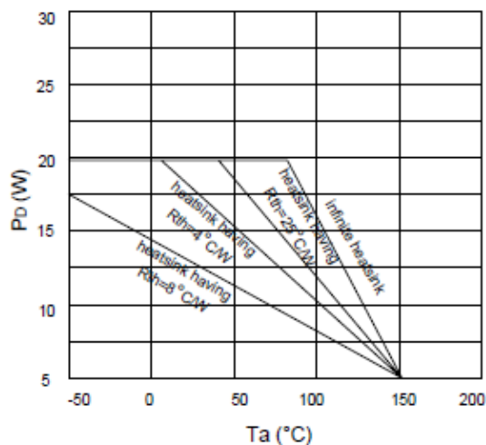
Fig.7 Maximum allowable power dissipation vs. ambient temperature
