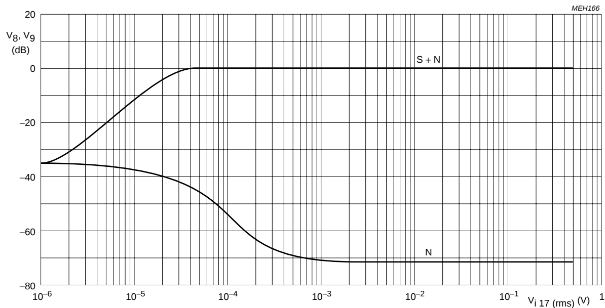
Fig.3 AF output voltage level on pins 8 and 9 as a function of V ilF at V P = 8.5 V; f m = 1 kHz; Q L = 20 with de-emphasis.
