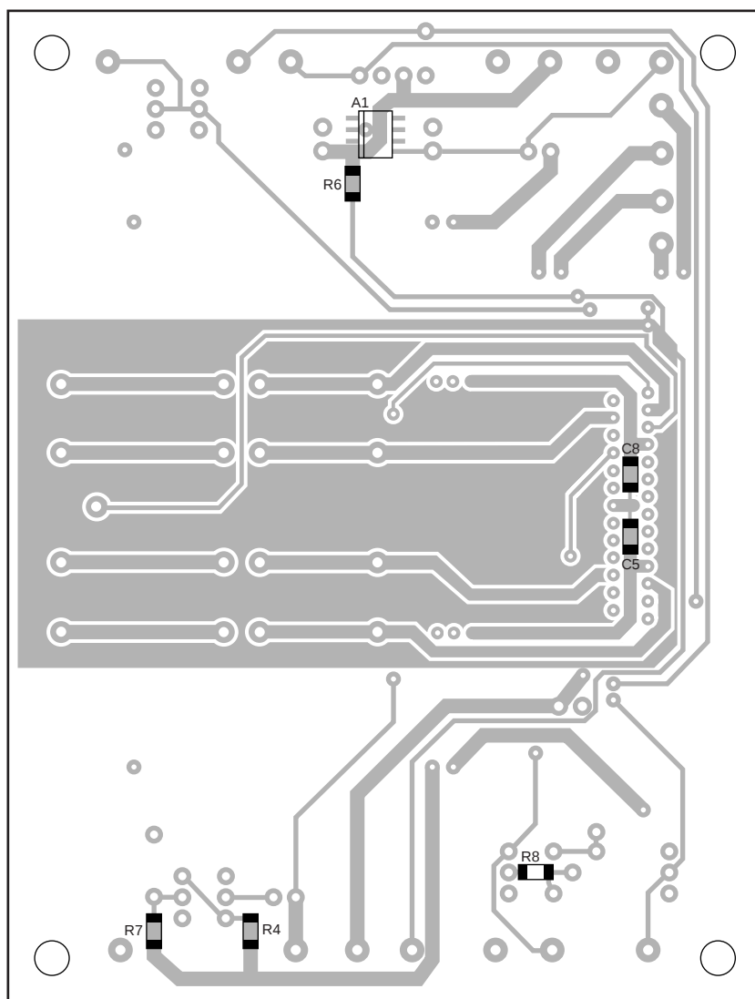
Fig 21. PCB layout TDA1566J, components bottom
