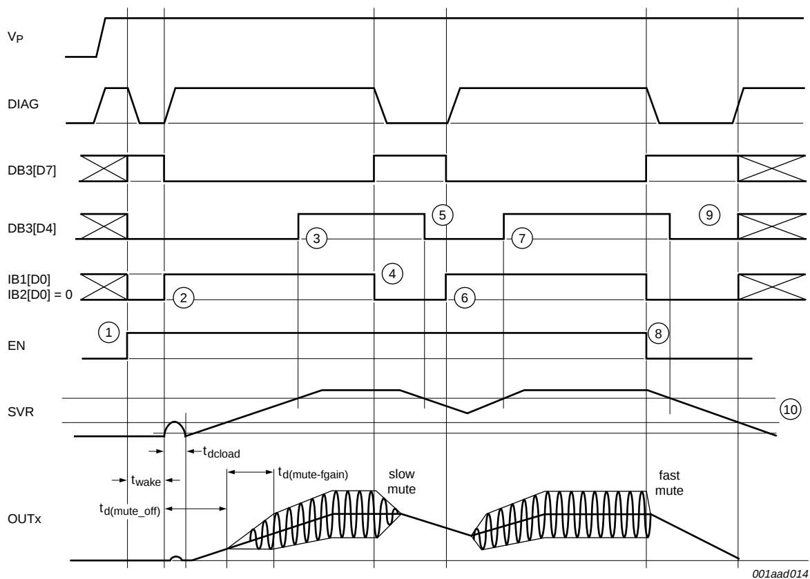
Fig 11. Start-up and shutdown timing in I 2 C-bus mode
