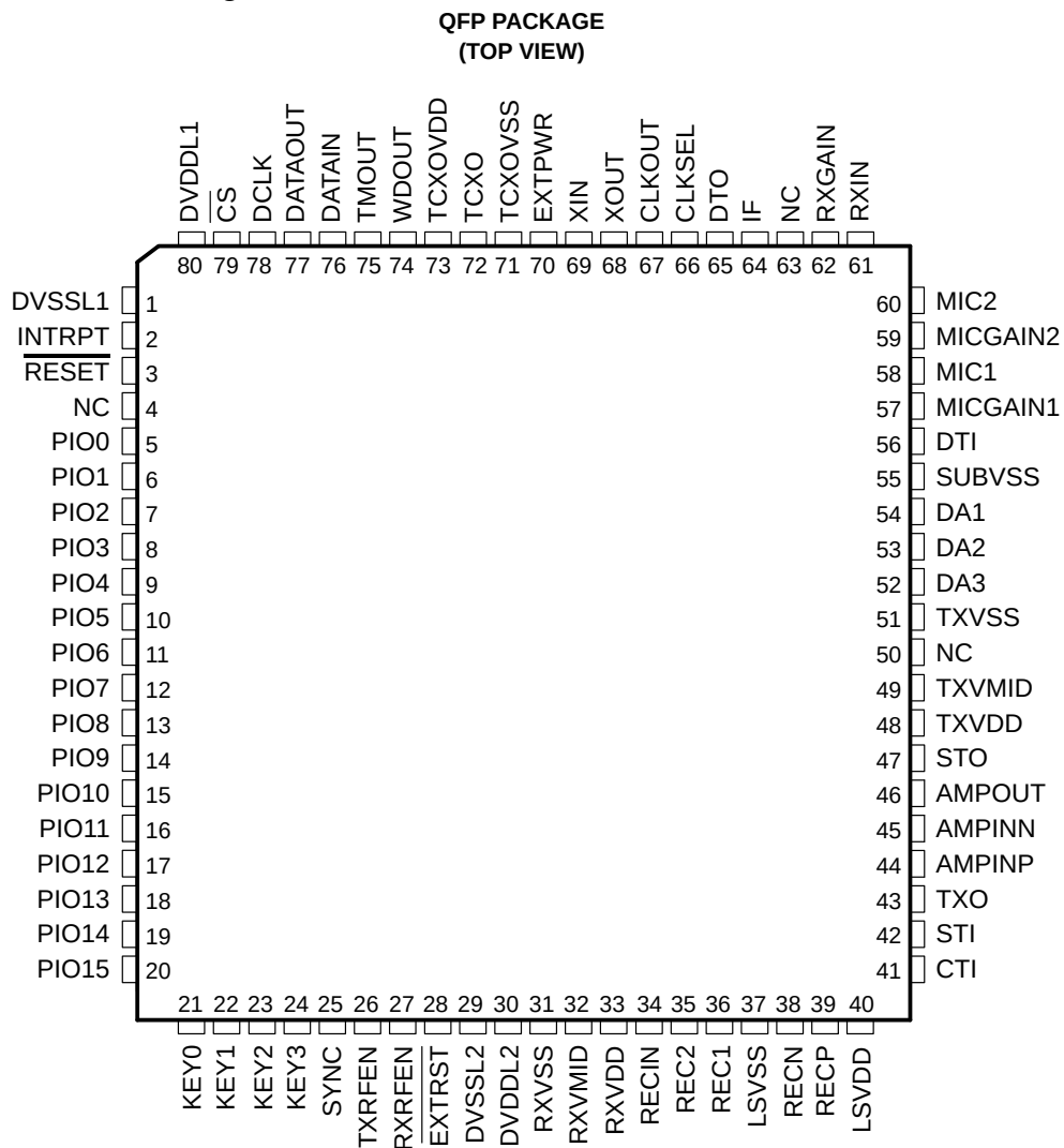
Figure 1-2. Terminal Assignments
