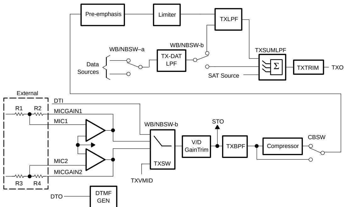
Figure 5–3. Transmit Audio Path
