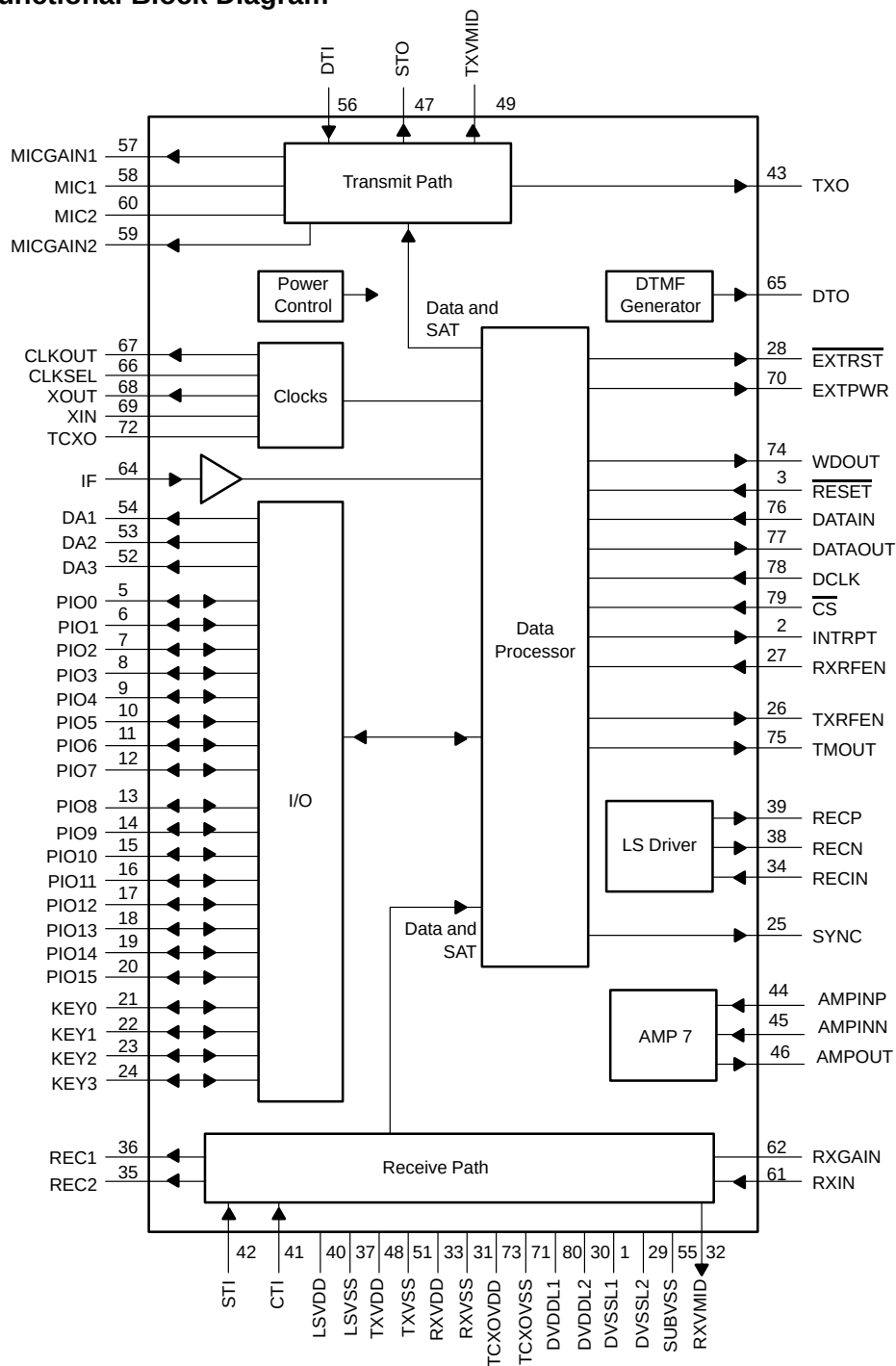
Figure 1-1. Functional Block Diagram
