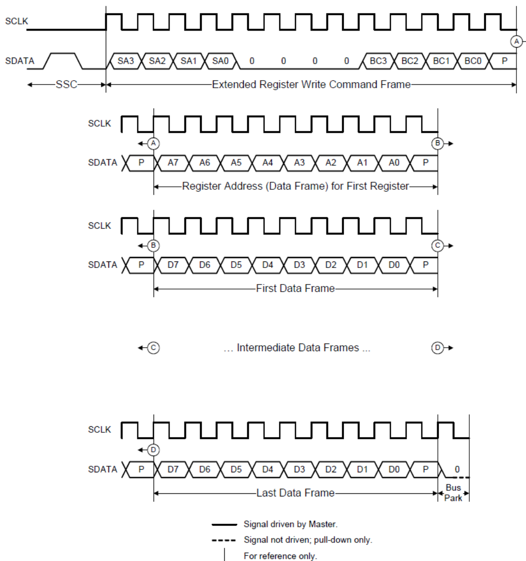
Figure 15. Extended Register Write Command Sequence
