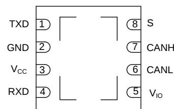
DRB Package for (V), (GV), (HV) and (HGV) Devices 8 PIN (VSON) Top View
