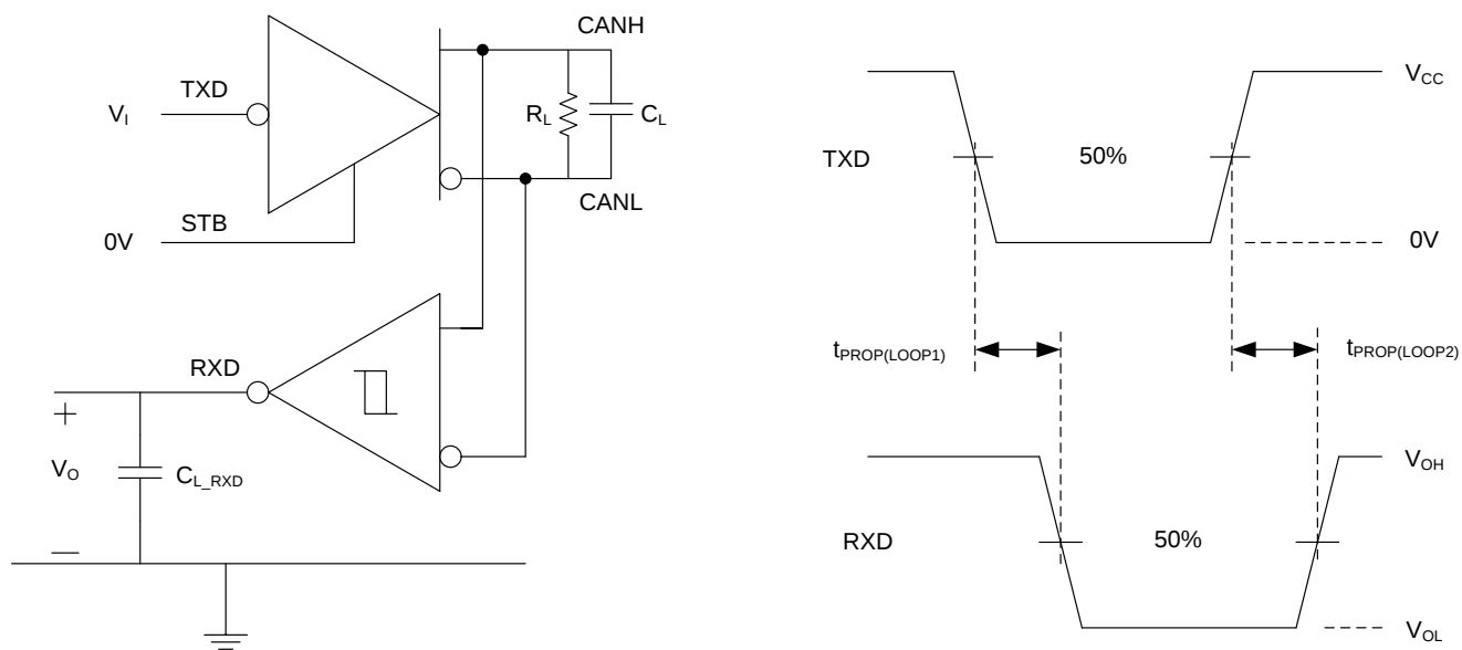
Figure 7. t_{\text{MODE}} Test Circuit and Measurement
