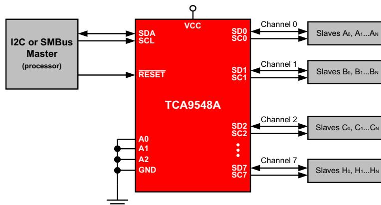
Simplified Application Diagram
