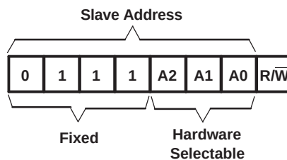
Figure 17. TCA9534A Address
