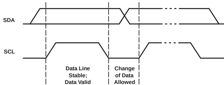
Figure 15. Bit Transfer
