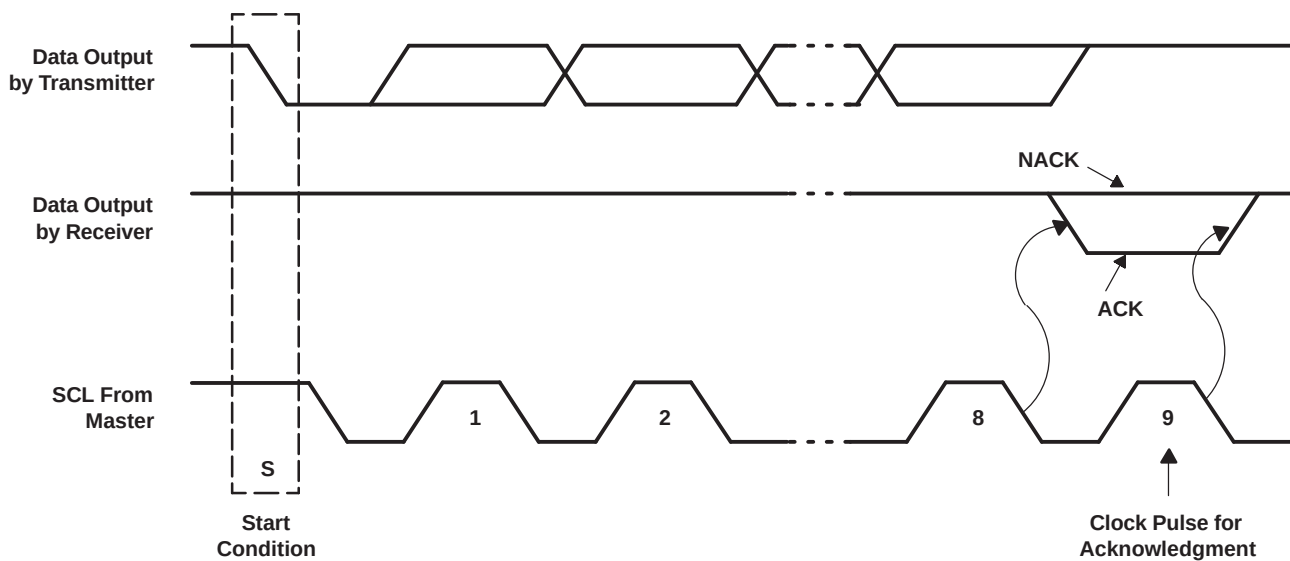
Figure 16. Acknowledgment on I²C Bus
