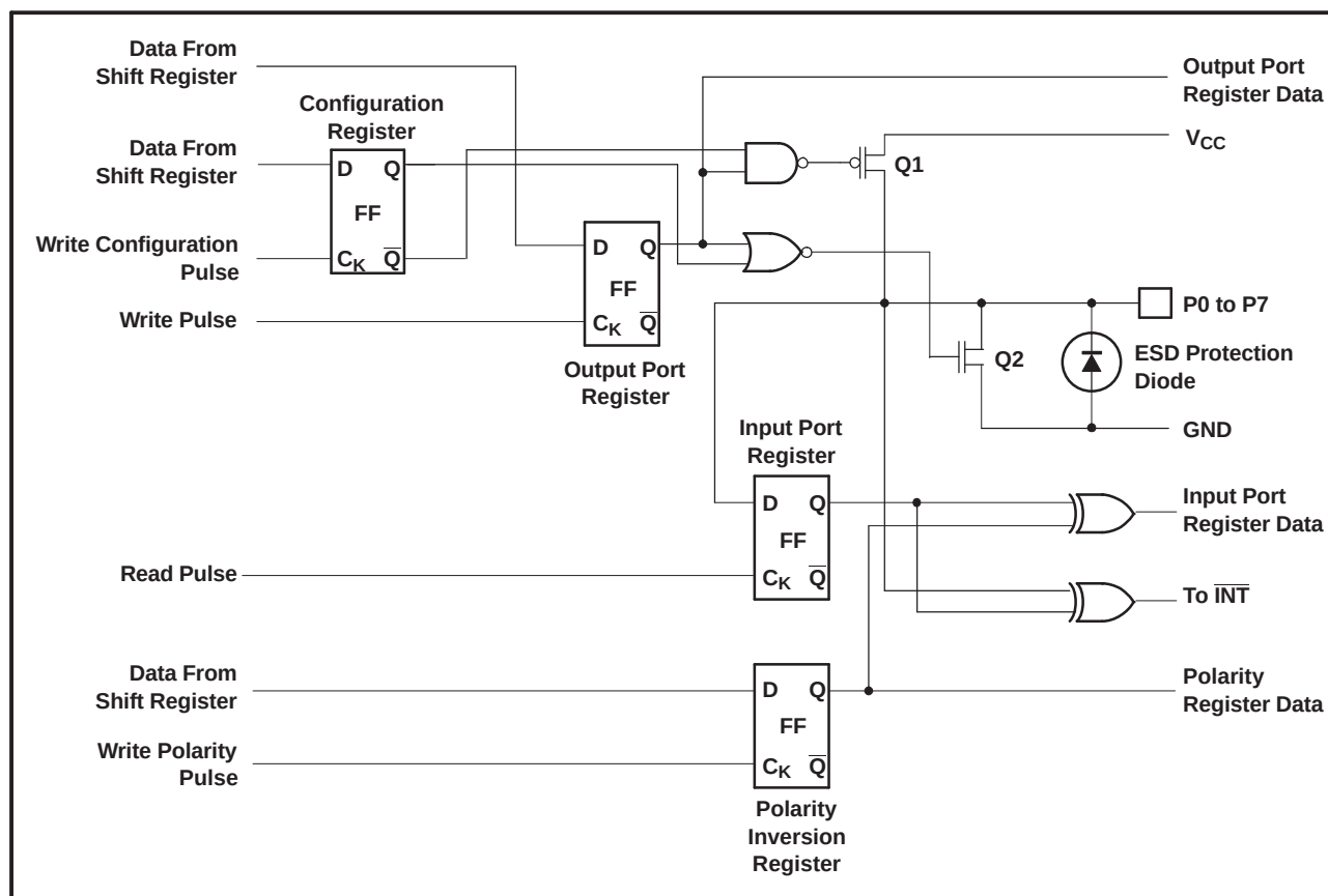
Figure 13. Simplified Schematic Of P0 To P7
