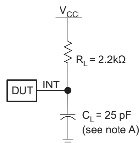
Figure 11. I²C Interface Load Circuit and Voltage Waveforms
