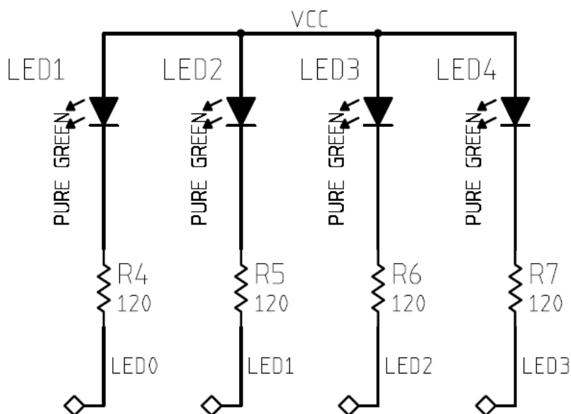
Figure 9. LED Outputs
