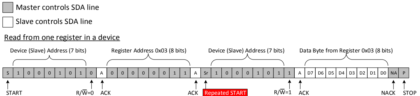
Figure 16. Read From Register Example
