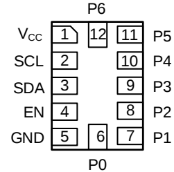
RUE Package 12-Pin X2QFN Top View
