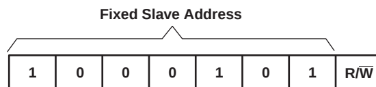
Figure 17. TCA6507 Address
