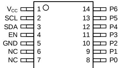
PW Package 14-Pin TSSOP Top View
