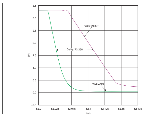
Figure 10. Input-Output Connection t_{PLH}
