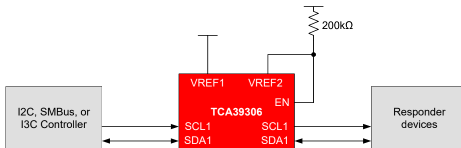
Simplified Application Diagram
