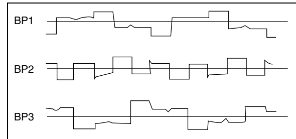
FIGURE 5-13: Backplane Waveforms.
