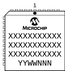
44-Pin PLCC
