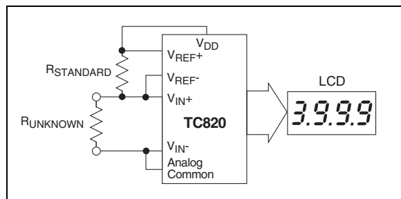
FIGURE 5-8: Low Parts Count Ratiometric Resistance Measurement.
