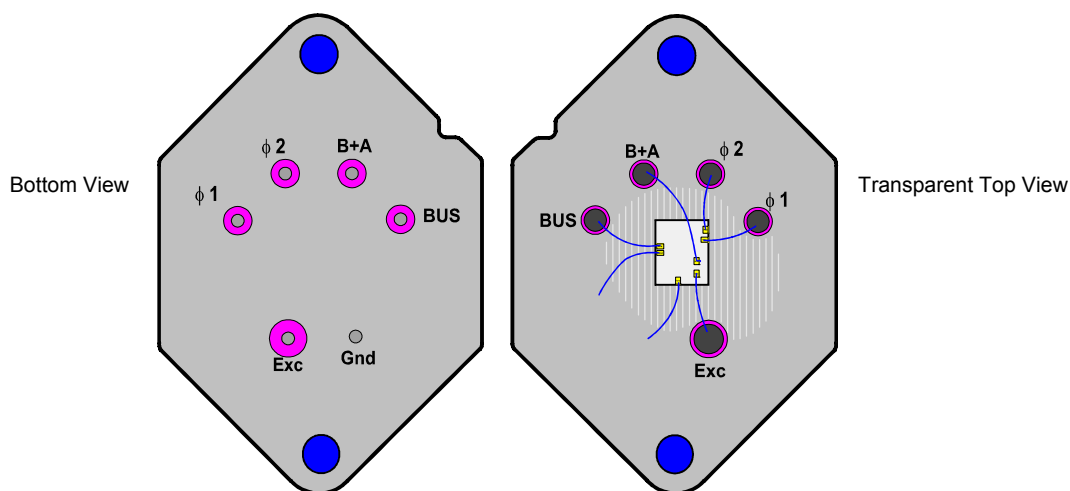
Figure 5. JTO3 pin connections (sample configuration only) non-production
