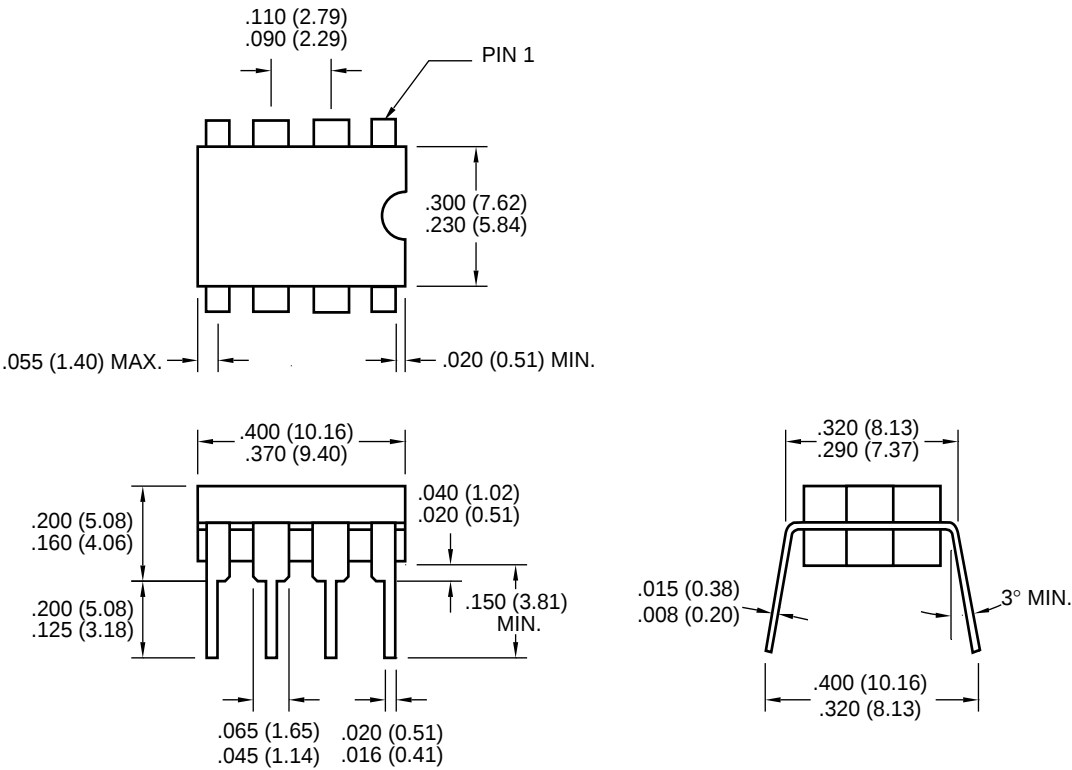
8-Pin Plastic DIP
