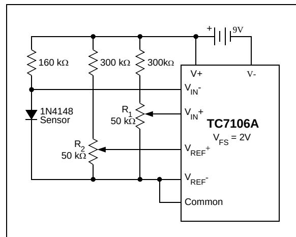
FIGURE 10-3: Temperature Sensor.
