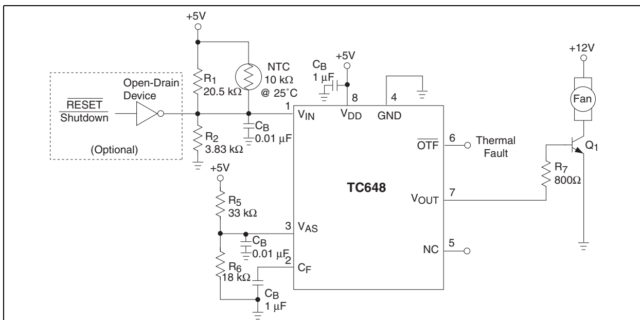
FIGURE 5-8: Design Example.
