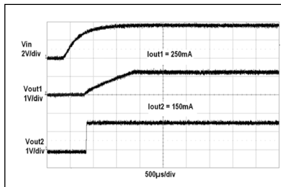
FIGURE 2-34: V_{OUT1} and V_{OUT2} Startup Waveforms.
