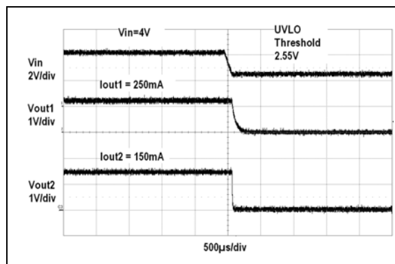
FIGURE 2-35: V_{OUT1} and V_{OUT2} Shutdown Waveforms.
