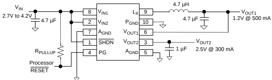
TC1304 Fixed-Output Application 10-Lead MSOP
