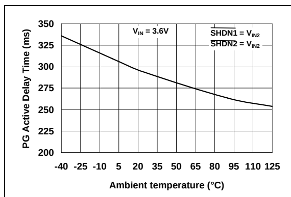
FIGURE 2-29: PG Active Delay Time-out vs. Ambient Temperature.
