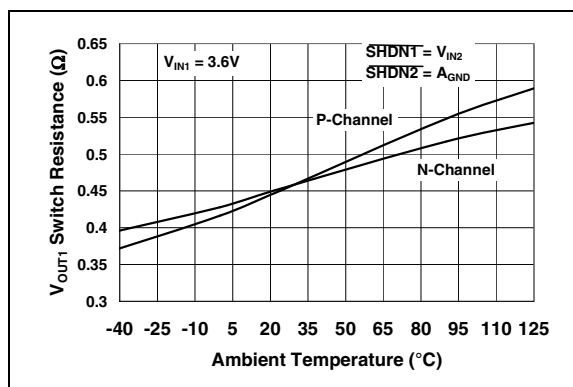
FIGURE 2-17: Buck Regulator Switch Resistance vs. Ambient Temperature.
