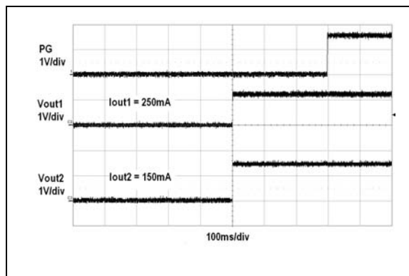
FIGURE 2-40: Power-Good Output Timing.
