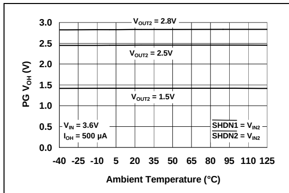
FIGURE 2-32: PG Output Voltage Level High vs. Ambient Temperature.
