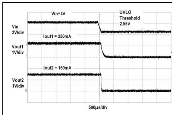
FIGURE 2-39: V_{OUT1} and V_{OUT2} Shutdown Waveforms.
