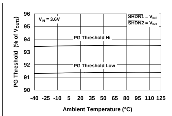
FIGURE 2-30: PG Threshold Voltage vs. Ambient Temperature.
