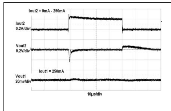
FIGURE 2-36: V_{OUT2} Load Step Response vs. Time.
