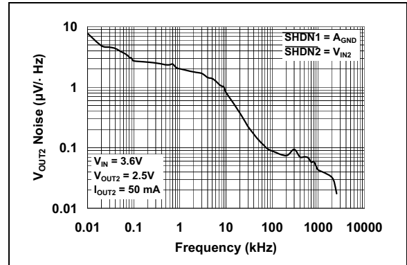
FIGURE 2-34: V_{OUT2} Noise vs. Frequency.
