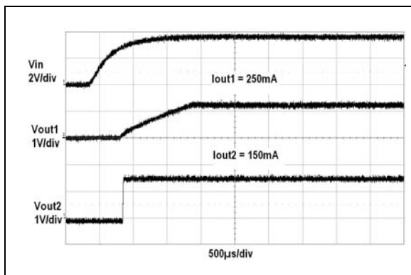
FIGURE 2-38: V_{OUT1} and V_{OUT2} Startup Waveforms.
