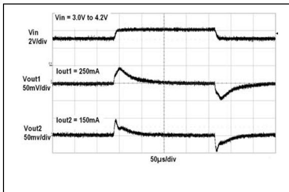
FIGURE 2-37: V_{OUT1} and V_{OUT2} Line Step Response vs. Time.
