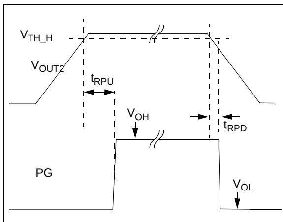
FIGURE 4-1: Power-Good Timing.
