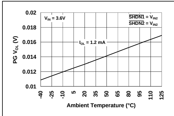
FIGURE 2-31: PG Output Voltage Level Low vs. Ambient Temperature.
