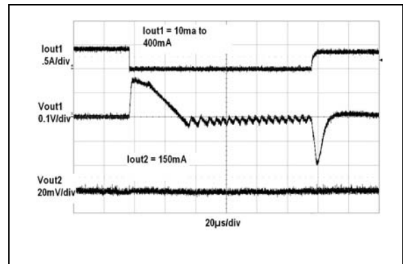
FIGURE 2-35: V_{OUT1} Load Step Response vs. Time.
