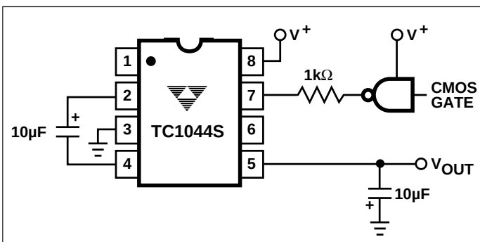
Figure 6. External Clocking
