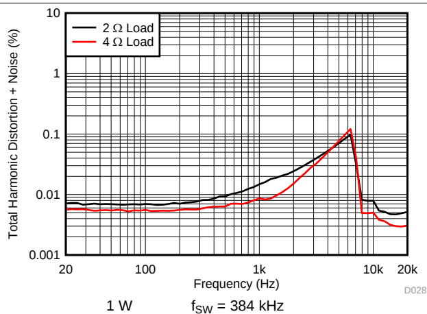
Figure 23. PBTLD THD+N vs Frequency
