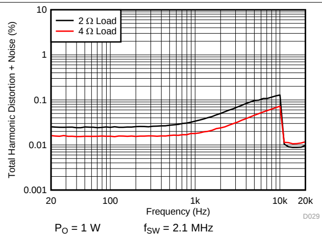
Figure 24. PBTLD THD+N vs Frequency
