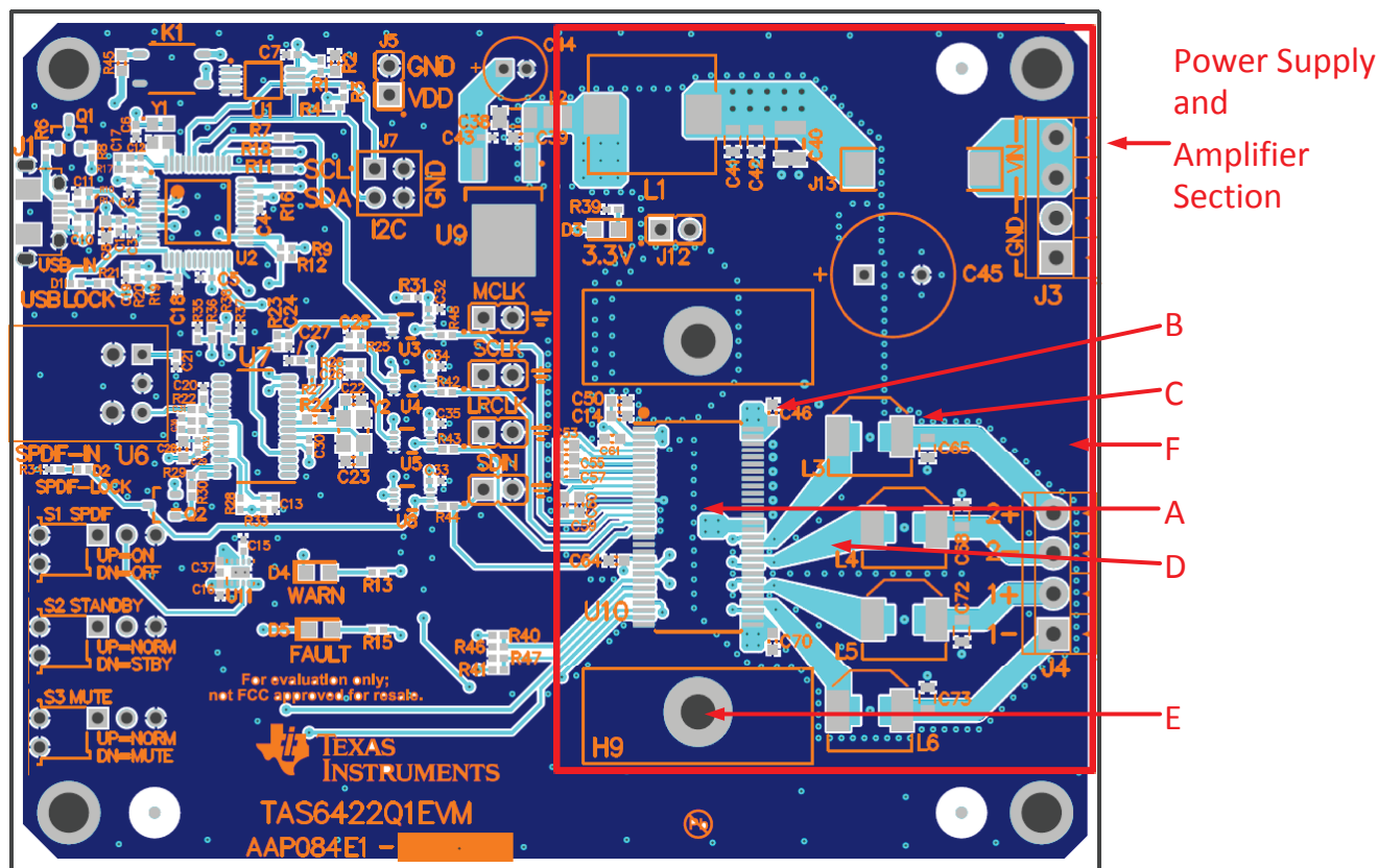
Figure 80. EVM Layout
