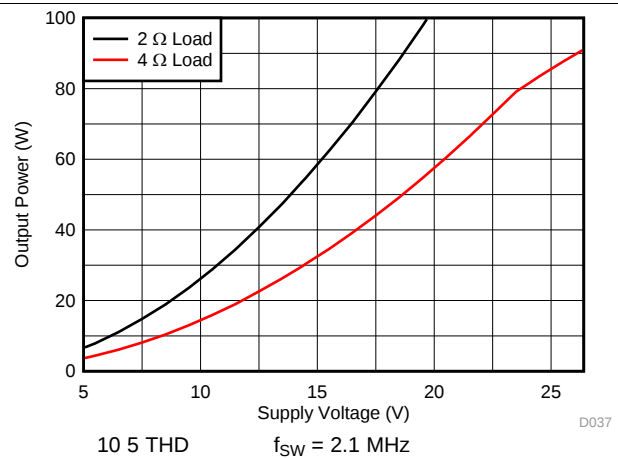
Figure 32. PBTl Output Power vs Voltage
