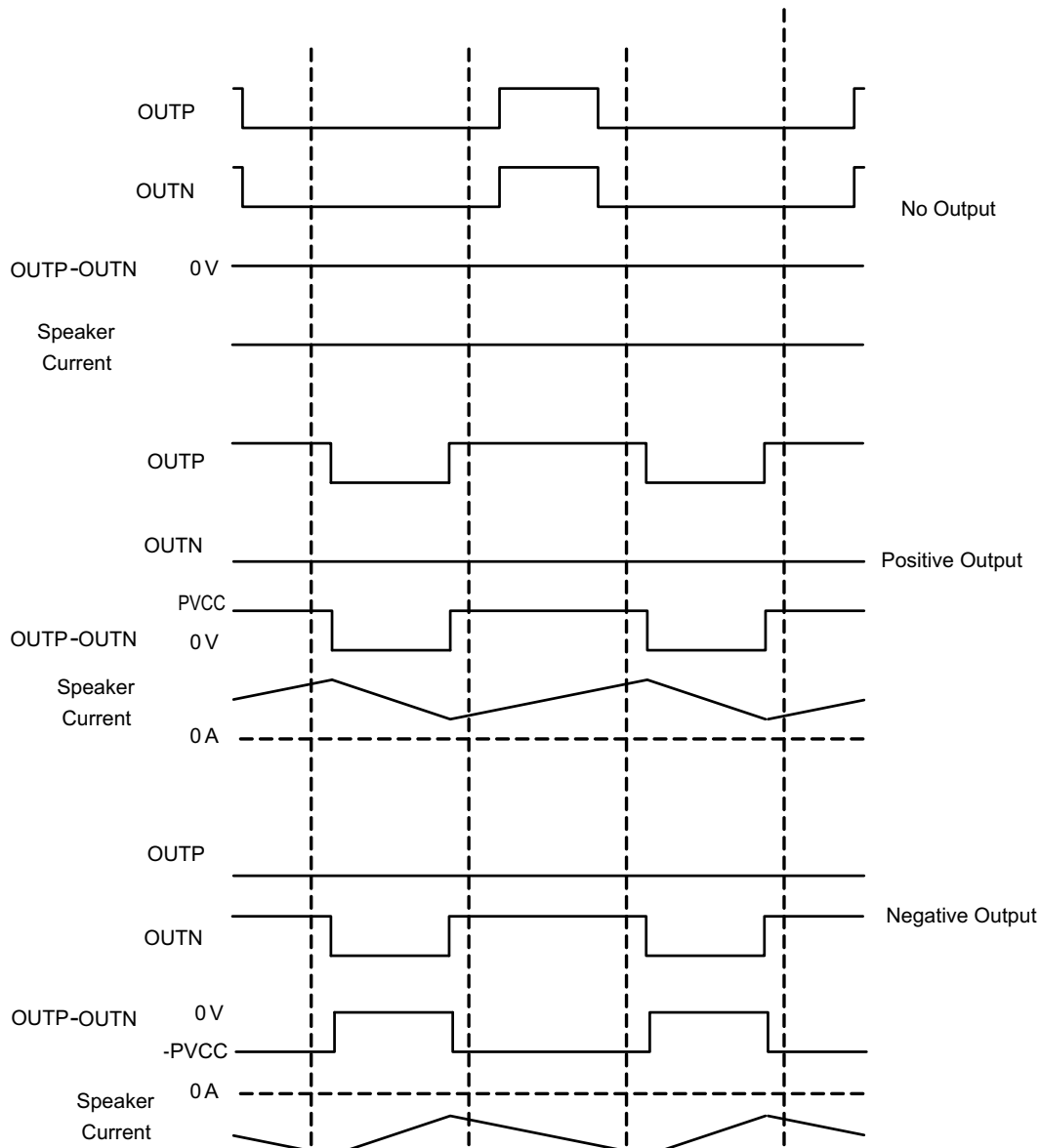
Figure 92. 1SPW Mode Modulation
