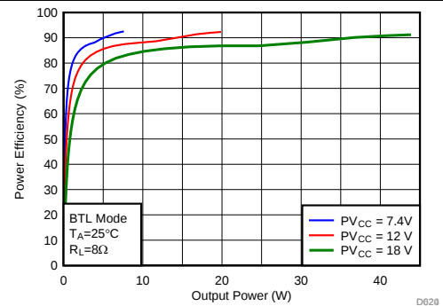
Figure 51. Efficiency vs Output Power
