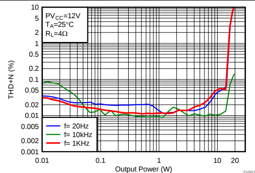
Figure 67. THD+N vs Output Power-PBTTL
