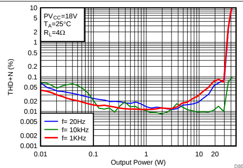
Figure 152. THD+N vs Output Power (Inductor as Output Filter, Hybrid Modulation, PBTL mode)
