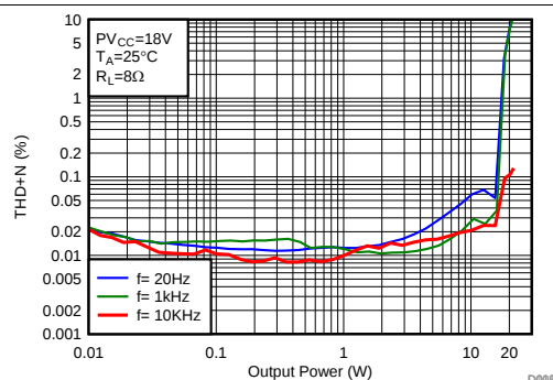
Figure 20. THD+N vs Output Power-BTL
