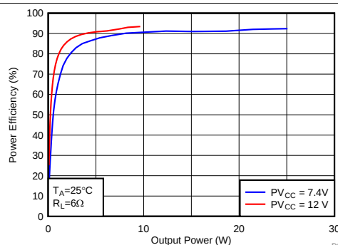
Figure 61. Efficiency vs Output Power-BTL
