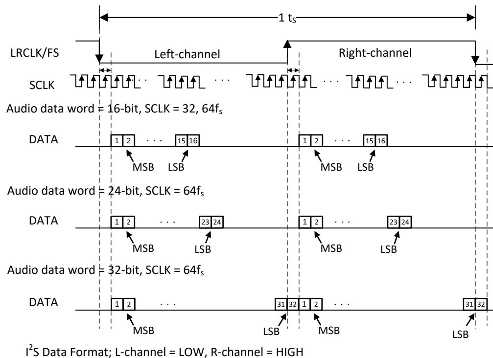
Figure 86. I^2S Audio Data Format
