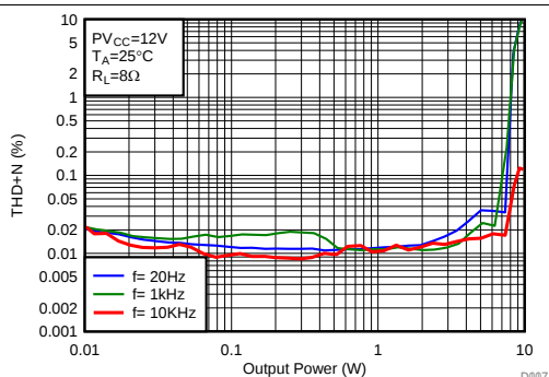
Figure 19. THD+N vs Output Power-BTL
