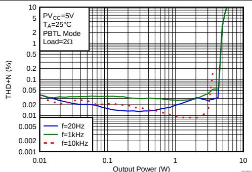
Figure 77. THD+N vs Output Power
