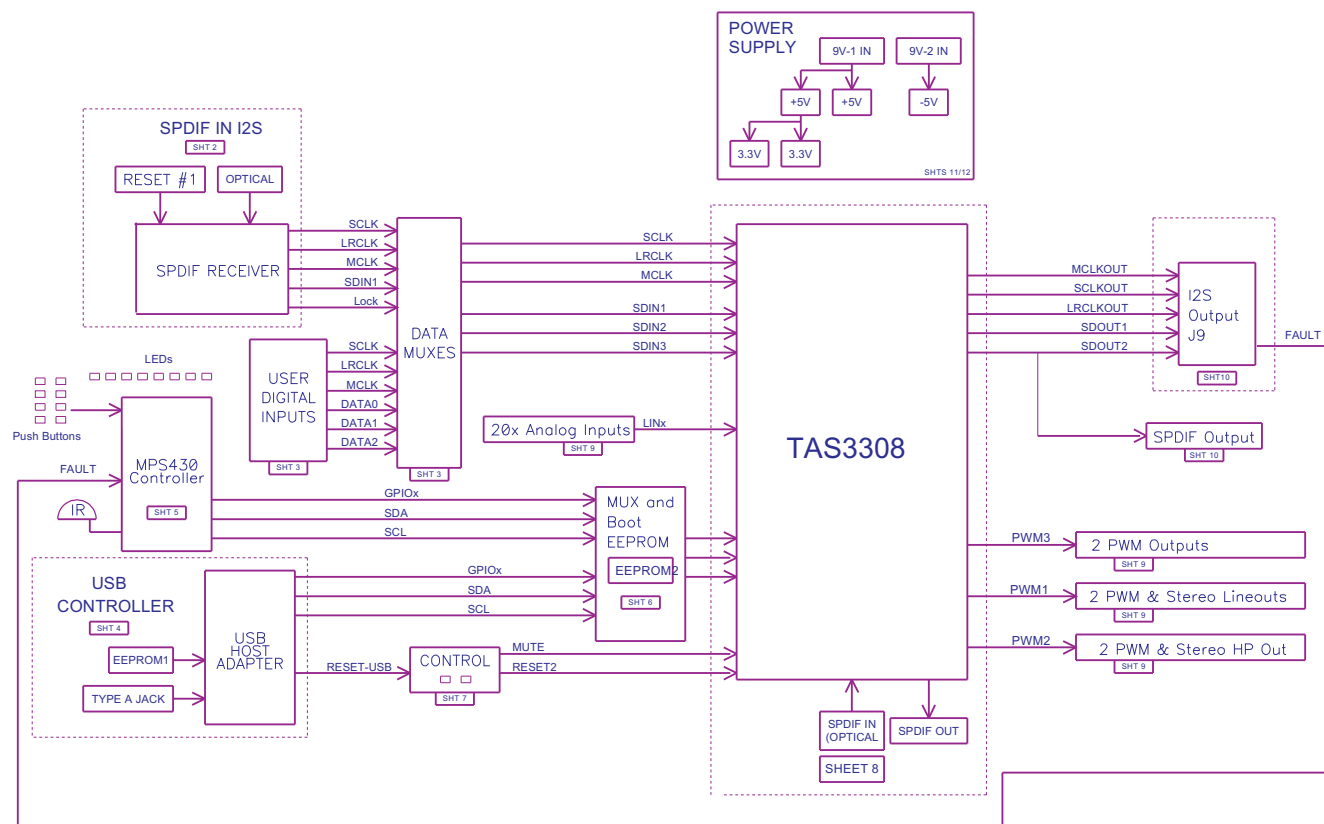
Figure 1-2. TAS3308EVM System
