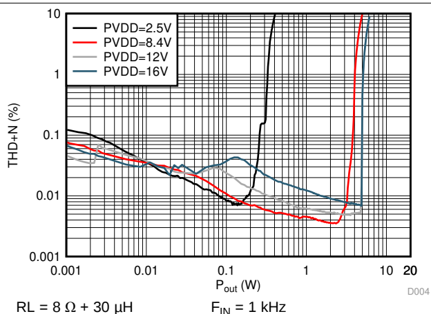
Figure 8. THD+N vs Output Power
