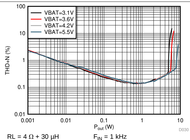
Figure 31. I-sense THD+N vs Output Power
