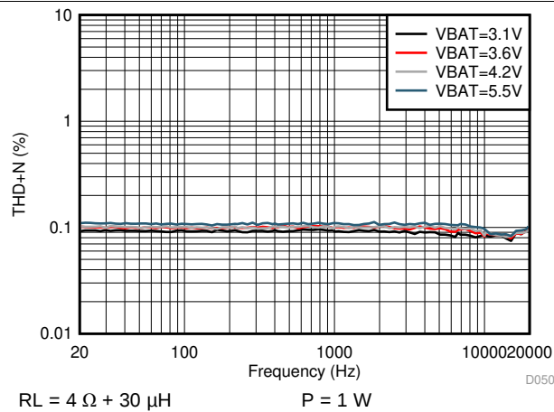
Figure 41. V-sense THD+N vs Frequency
