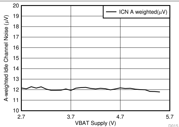
Figure 17. Idle Channel Noise (A-Weighted) vs VBAT
