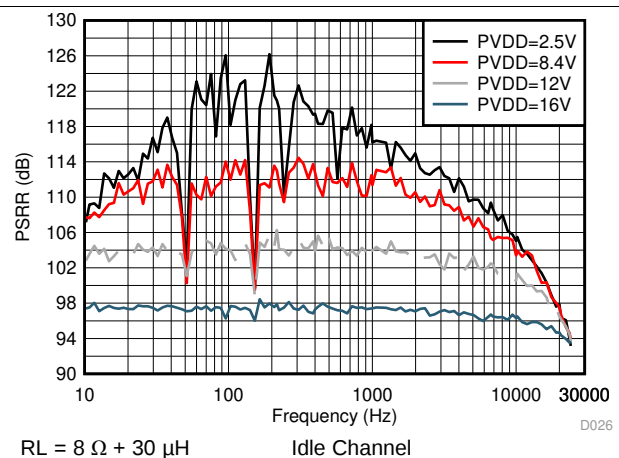
Figure 28. PVDD PSRR vs Frequency
