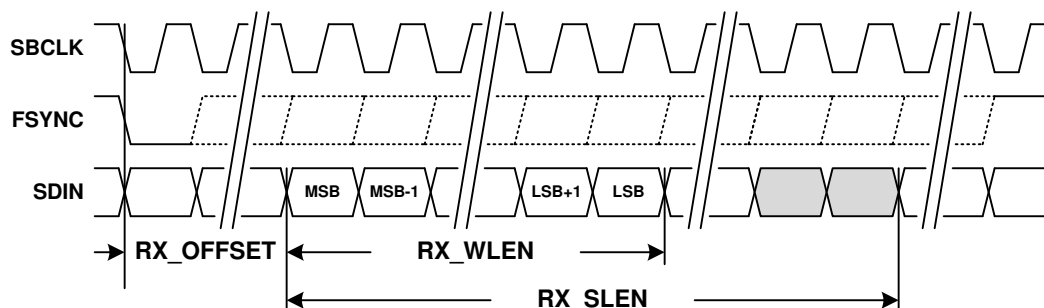
Figure 59. TDM RX Time Slot with Left Justification
