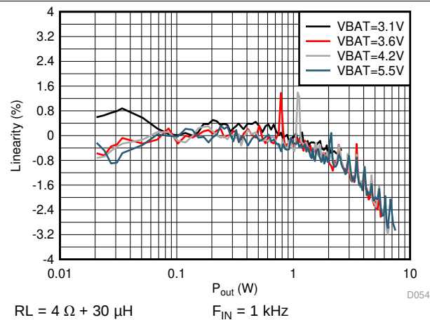
Figure 43. V/I-sense Linearity vs Output Power
