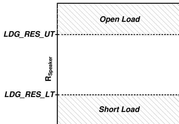
Figure 67. Load Diagnostics
