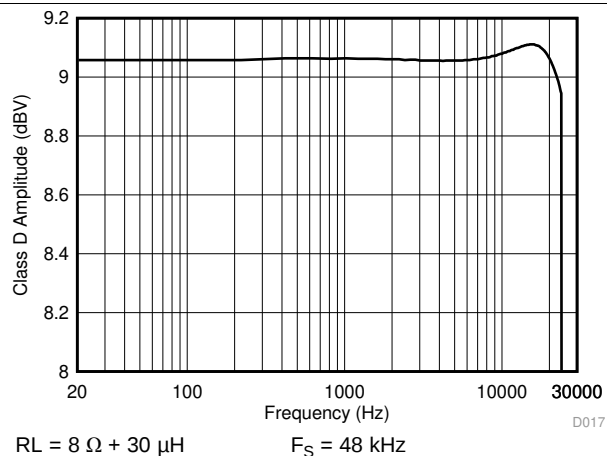
Figure 19. Amplitude vs Frequency
