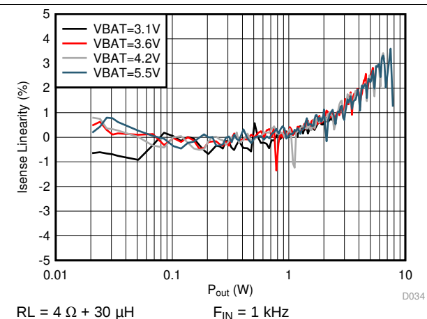
Figure 33. I-sense Linearity vs Output Power
