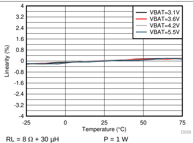
Figure 46. V-sense Linearity vs Temperature
