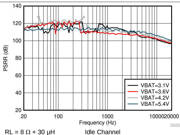
Figure 27. VBAT PSRR vs Frequency
