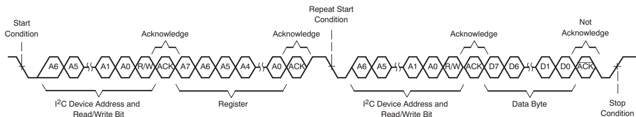
Figure 55. Single-Byte Read Transfer
