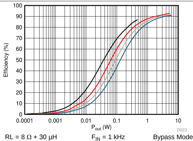
Figure 25. Efficiency vs Output Power
