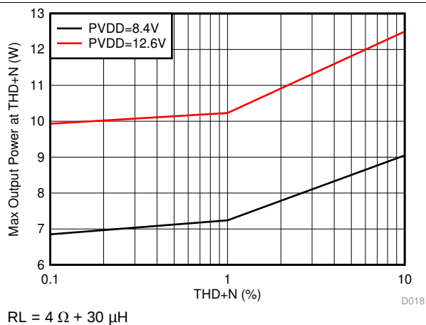
Figure 20. Max Output Power vs THD+N
