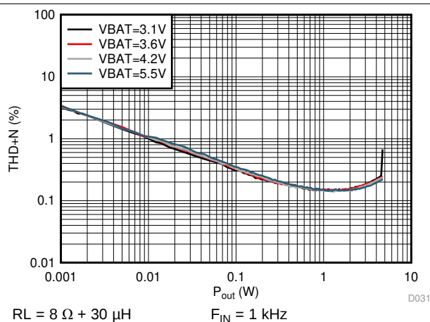
Figure 32. I-sense THD+N vs Output Power
