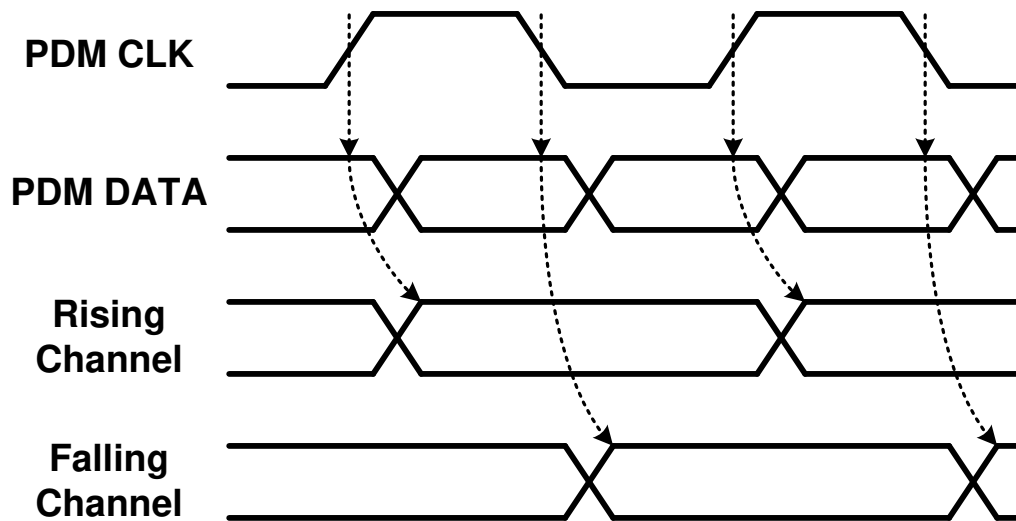
Figure 58. PDM Waveform
