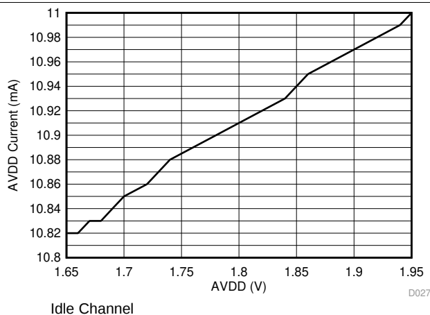
Figure 29. AVDD Idle Current vs AVDD
