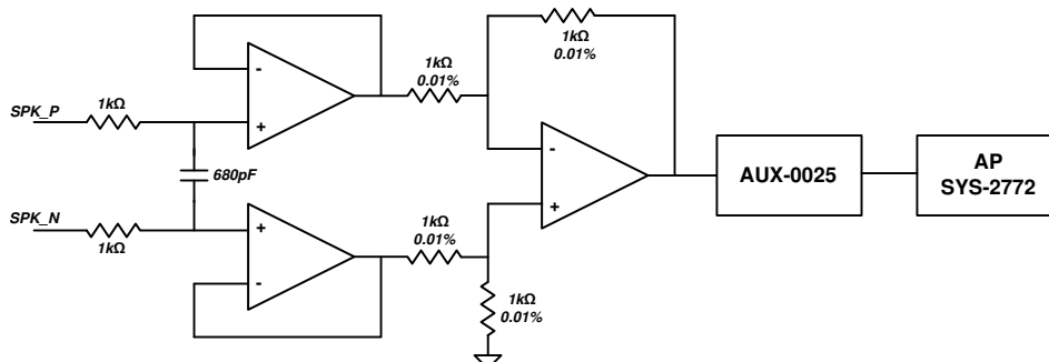
Figure 49. Differential To Single Ended (D2S) Filter
