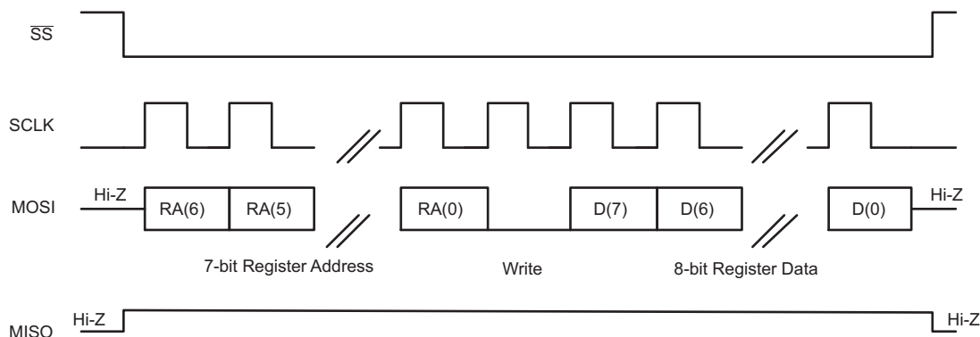
Figure 51. SPI Timing Diagram for Register Write
