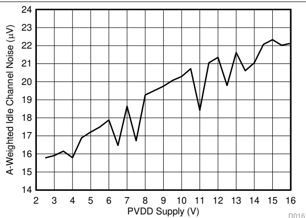
Figure 18. Idle Channel Noise (A-Weighted) vs PVDD
