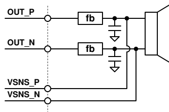
Figure 66. V-Sense Connections
