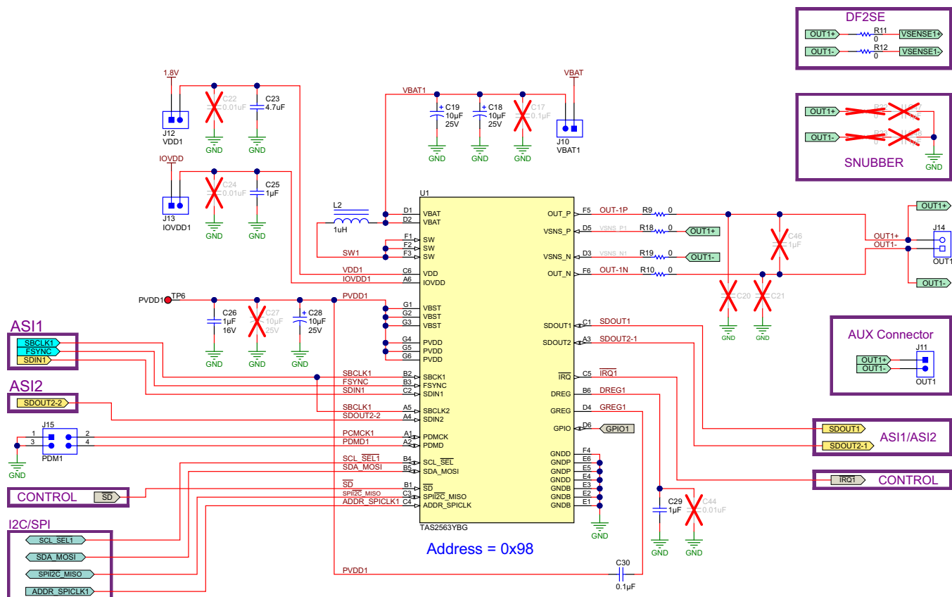
Figure 48. TAS2563 Circuit
