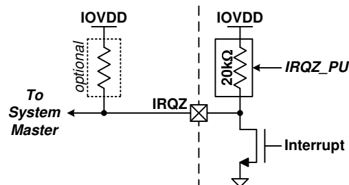
Figure 57. IRQZ Pin
