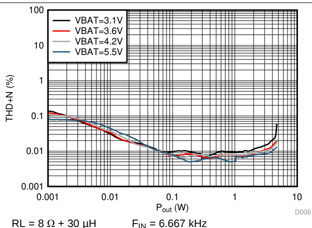
Figure 10. THD+N vs Output Power
