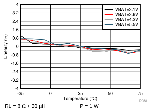
Figure 45. I-sense Linearity vs Temperature
