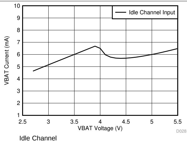
Figure 30. VBAT Idle Current vs VBAT
