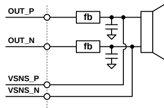
Figure 67. V-Sense Connections
