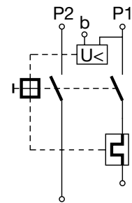
Mechanical lock-out latch
