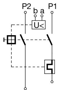
Undervoltage release with 2 additional contacts
