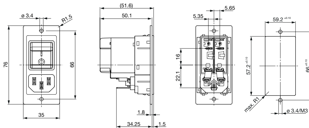
Screw-on mounting Version B for front mount IP40
