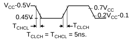
Figure 35. I_{CC} Test Condition, Power-Down Mode
