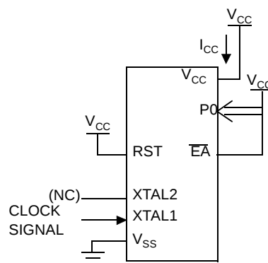
Figure 33. I_{CC} Test Condition, Active Mode
