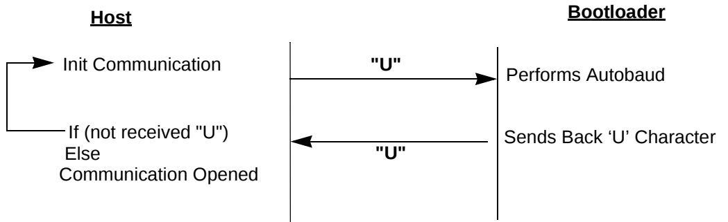
Figure 25. Initialization
