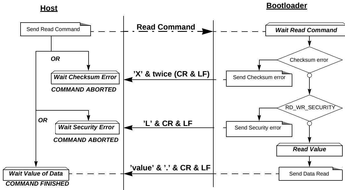
Figure 30. Read Flow
