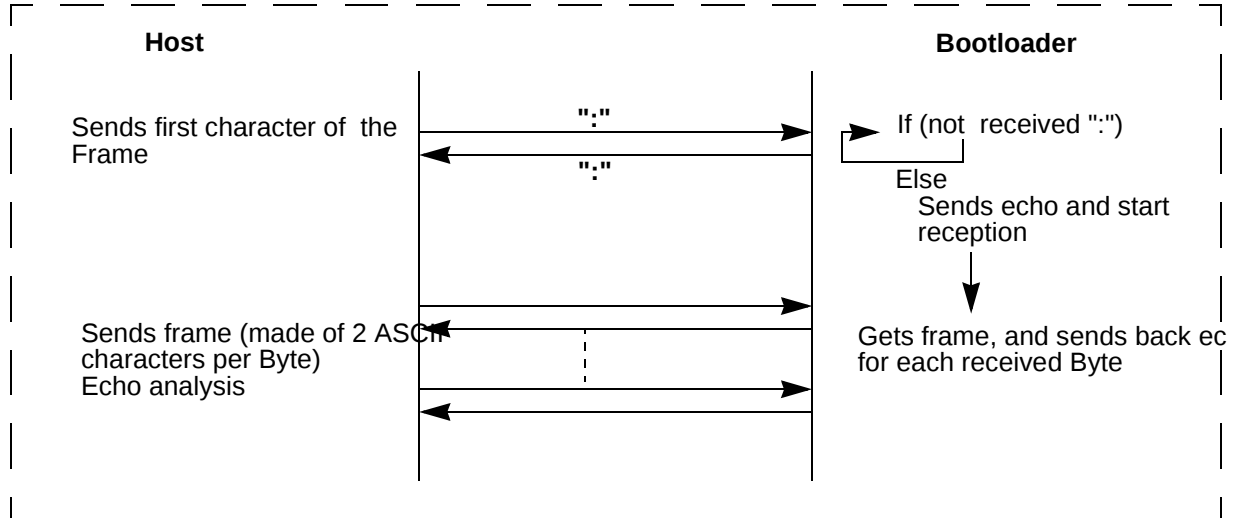
Figure 26. Command Flow
