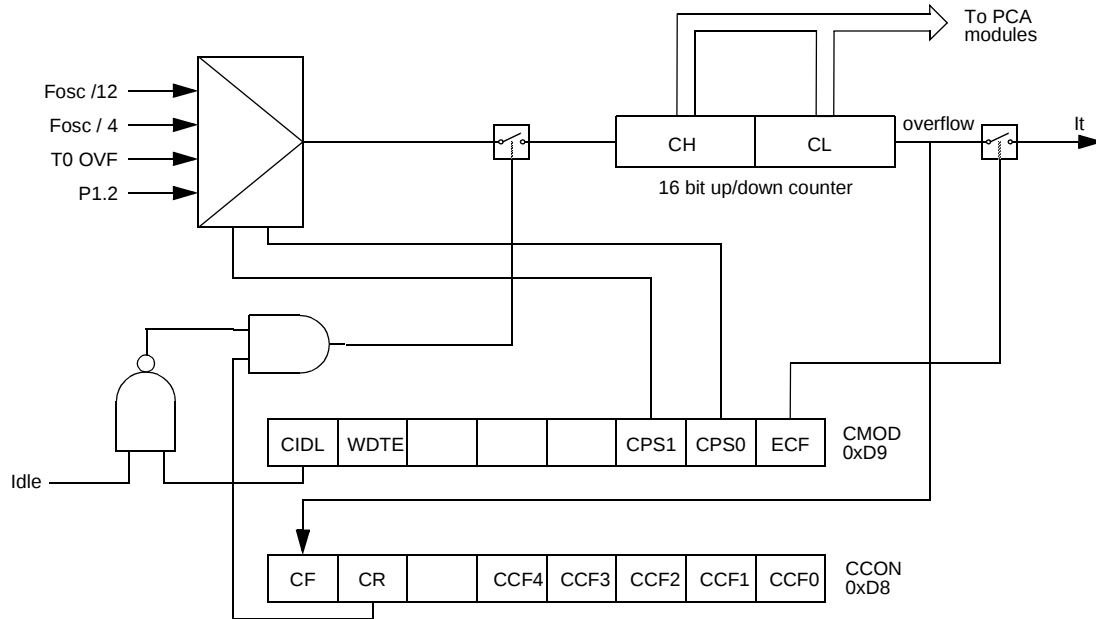
Figure 7. PCA Timer/Counter
