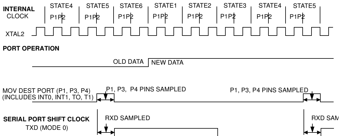
Figure 26. Clock Waveforms
