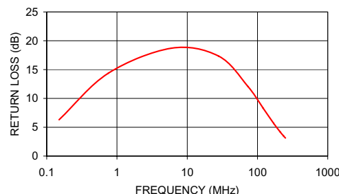
T8-1-X65 INPUT RETURN LOSS
