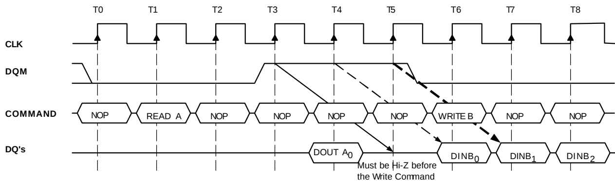
Read to Write Interval (Burst Length ≥ 4, CAS# Latency = 3)
