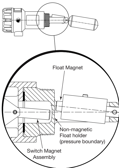
Figure 11 Magnet/Switch Action
