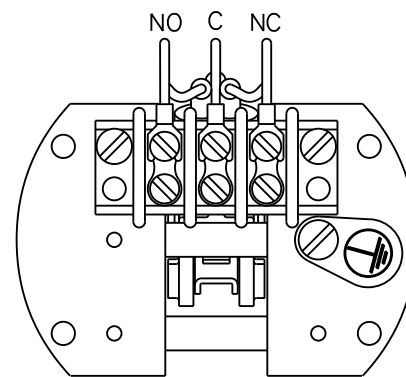
Figure 8 Terminal Connections SPDT HS switch with silver or gold contacts
