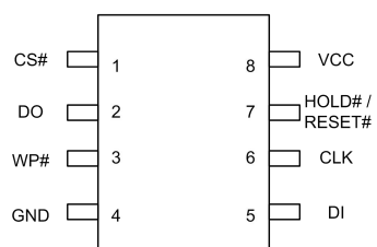
Figure 3.1 8-pin SOP (150/208mil)/ PDIP (300mil)
