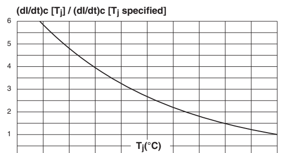
Figure 10. Relative variation of critical rate of decrease of main current versus T_j
