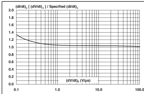
Figure 9. Relative variation of critical rate of decrease of main current (di/dt)_c versus reappplied (dV/dt)_c (typical values)
