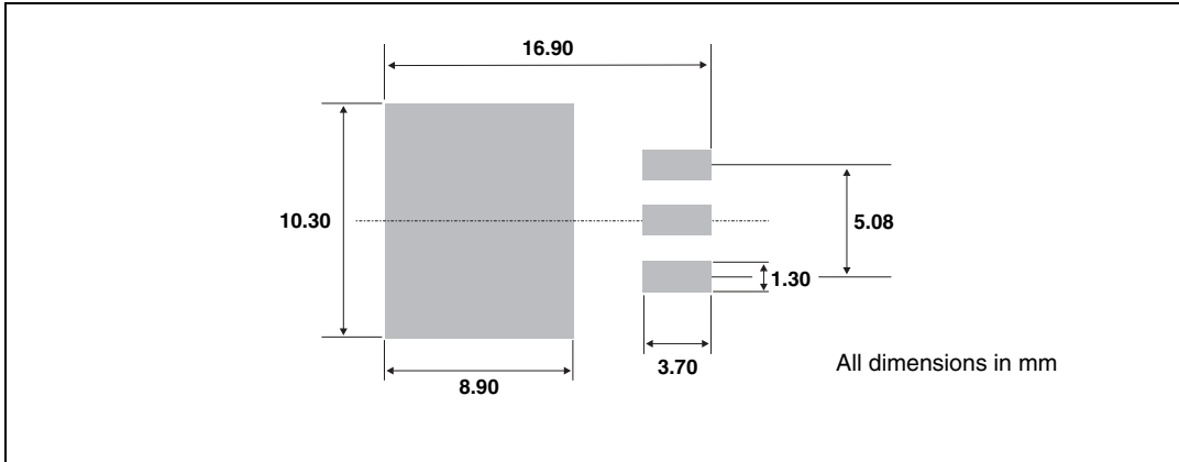
Figure 14. D 2 PAK Footprint
