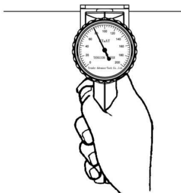
Fig 4.4 Read measurement
