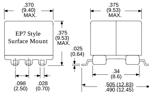
Package for T-531SM
