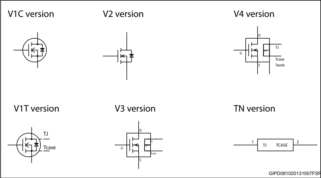
Figure 2. Model symbols
