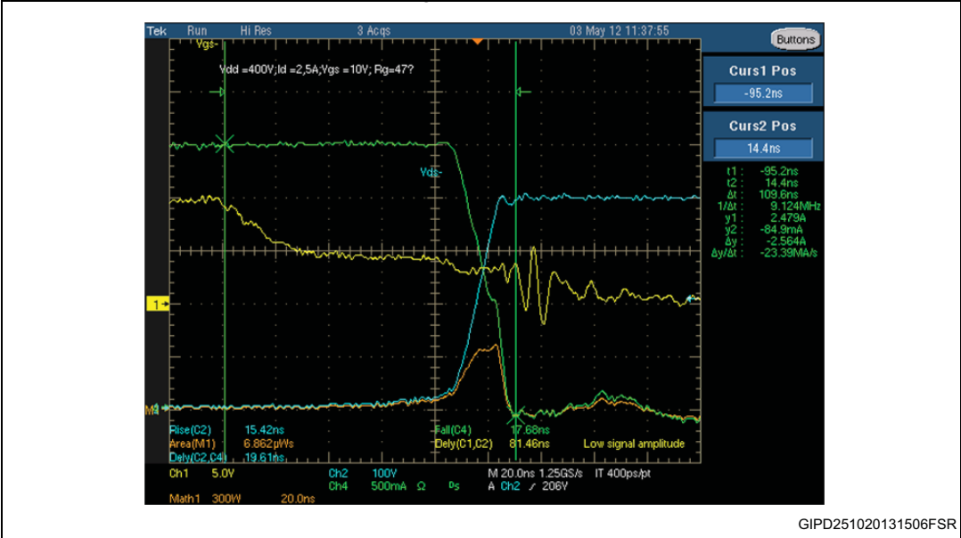
Figure 20. E_{off} vs R_{gate} - experimental waveforms
