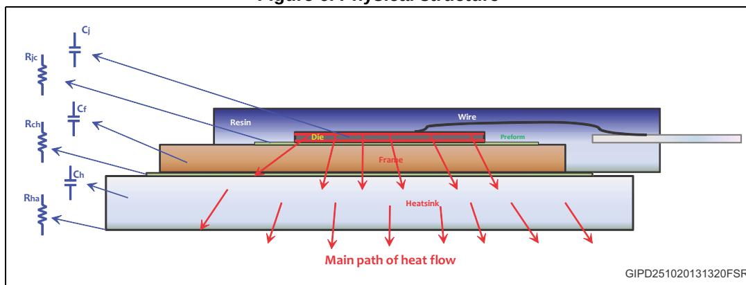
Figure 6. Physical structure
