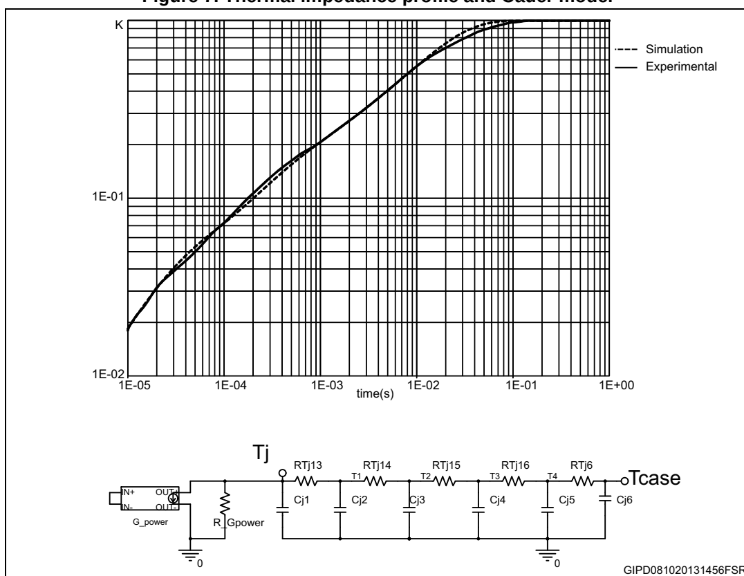
Figure 7. Thermal impedance profile and Cauer model
