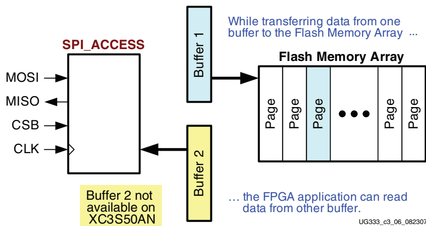
Figure 3-6: SRAM Page Buffers Support Read-while-Write Operations
