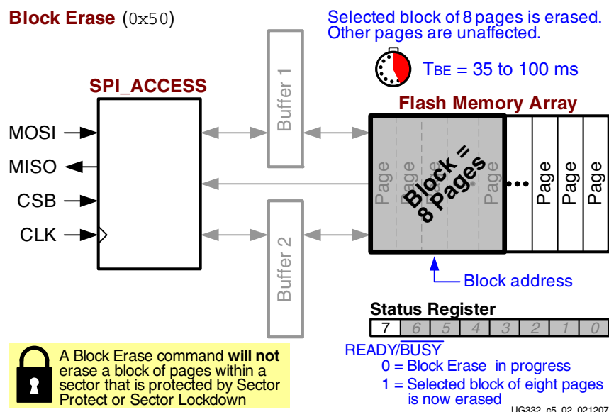
Figure 5-2: Block Erase Command
