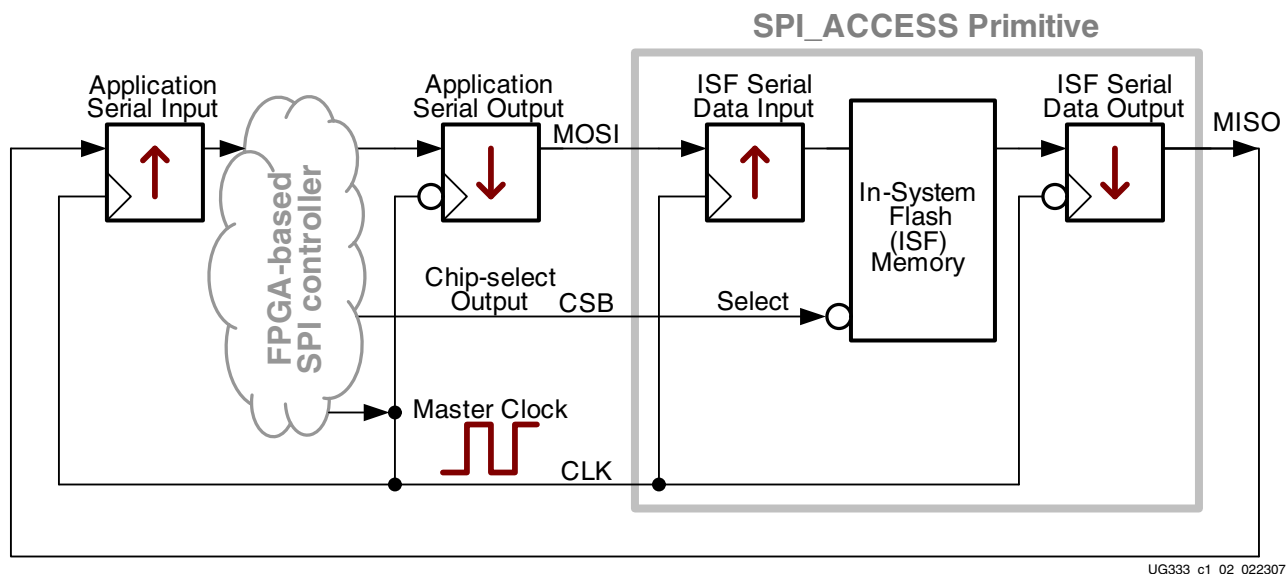
Figure 1-2: FPGA-to-SPI_ACCESS Interface and Active Clock Edges
