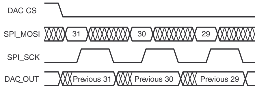
Figure 9-3: SPI Communication Waveforms
