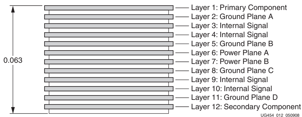
Figure 12: PCB Stackup
