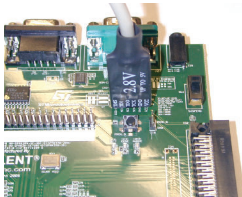
a) JTAG3 Parallel Connector
