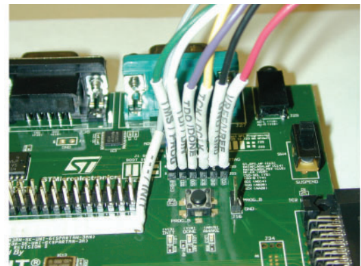
b) Parallel Cable III or Parallel Cable IV with Flying Leads
