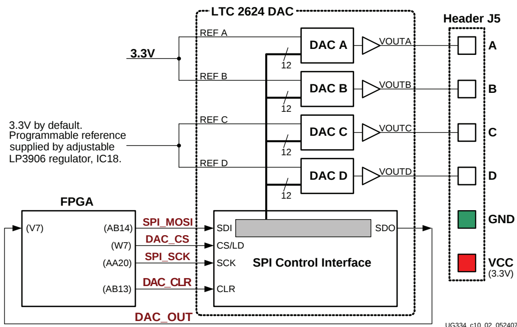
Figure 10-2: Digital-to-Analog Connection Schematics
