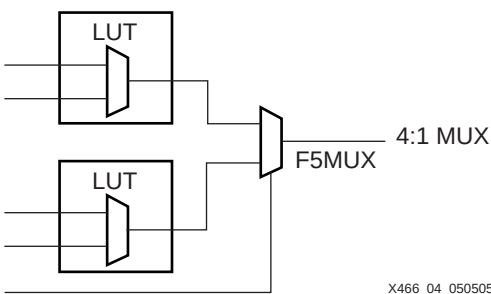
Figure 8-4: 4:1 Mux Implemented Using F5MUX
