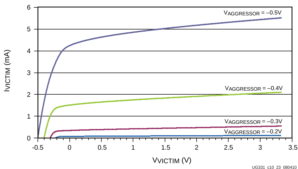
Figure 10-40: Figure Parasitic Leakage Across Different V_{\text{AGGRESSOR}} at 85°C
