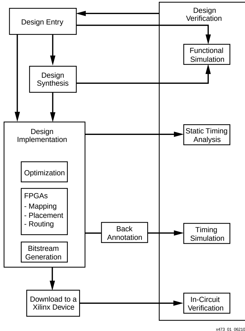
Figure 13-1: Design Flow
