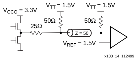
Figure 10-27: Terminated SSTL3 Class II
