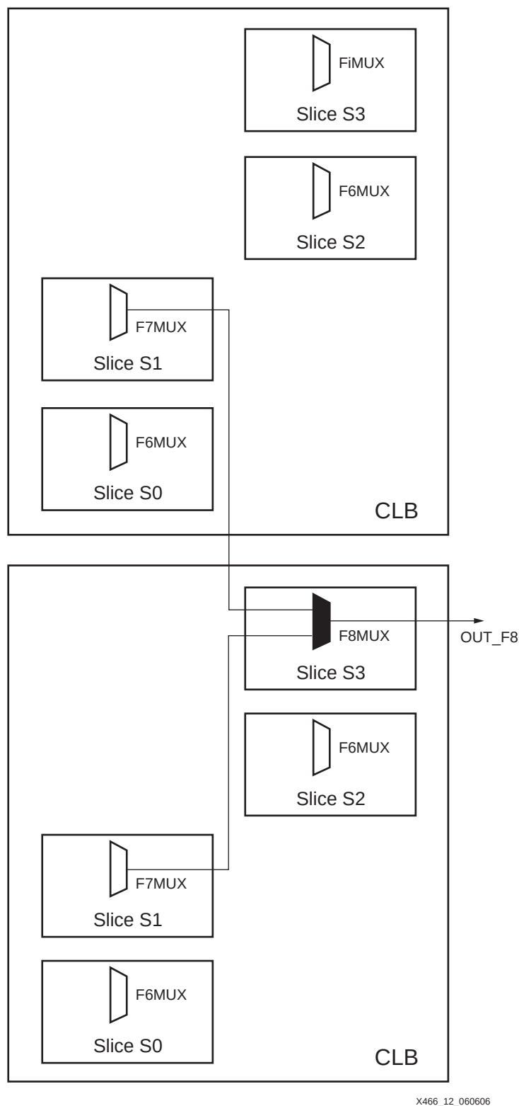
Figure 8-13: 79-input Function Using F8MUX in Two Adjacent CLBs
