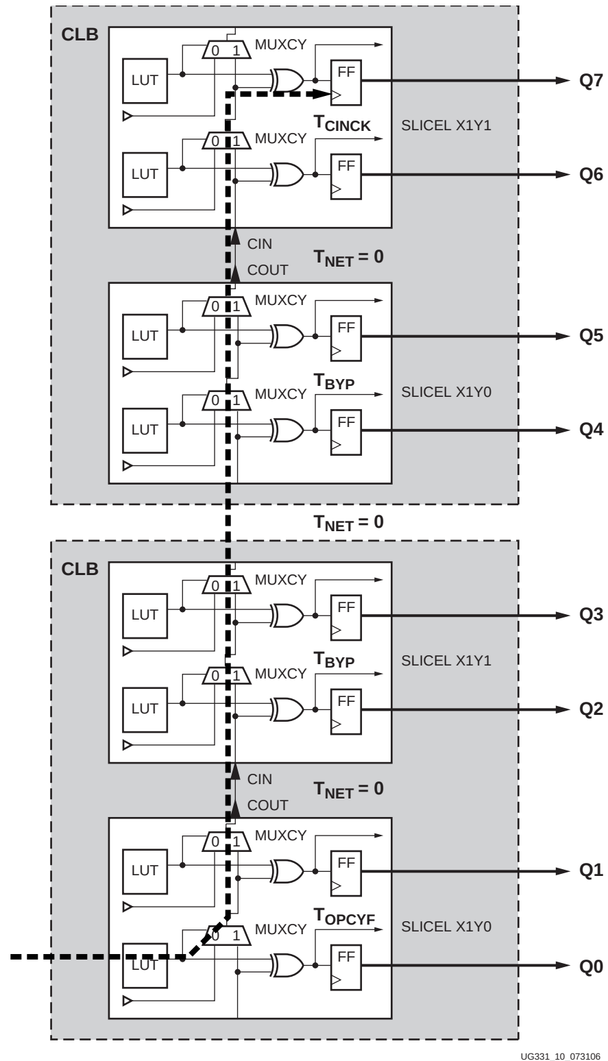
Figure 9-10: Carry Delay Path
