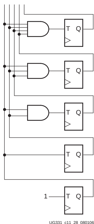
Figure 9-28: Binary Counter
