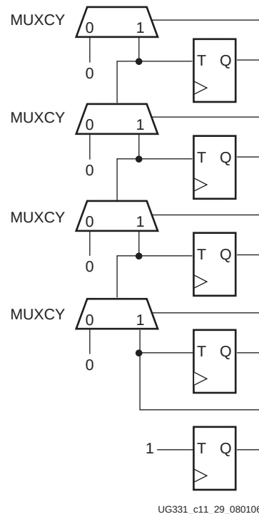
Figure 9-29: Binary Counter Using MUXCY for AND Gates
