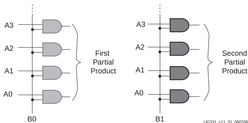
Figure 9-31: Partial Product Generation
