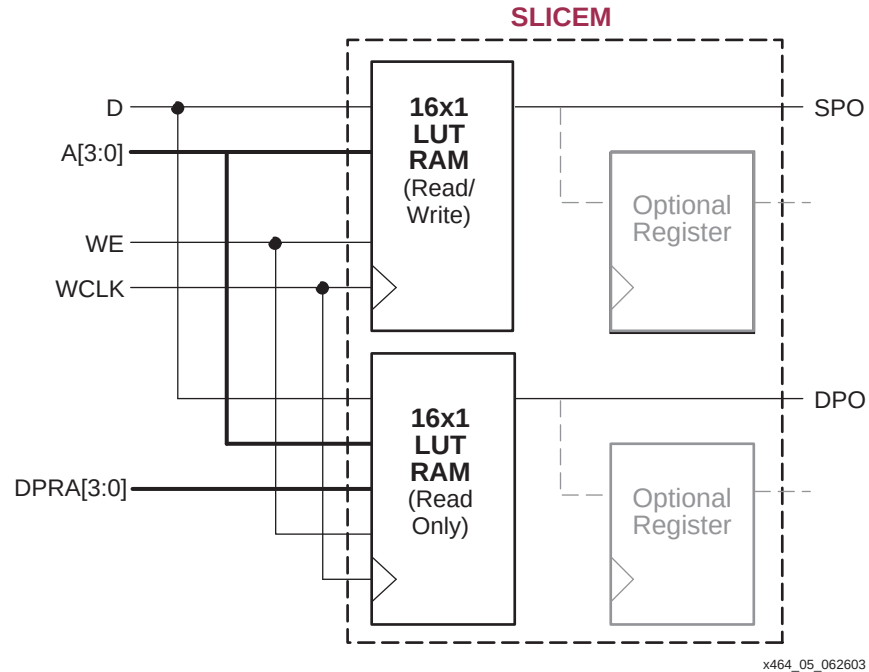
Figure 6-5: RAM16X1D Placement
