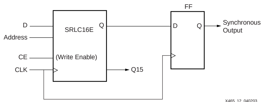
Figure 7-13: Fully Synchronous Shift Register
