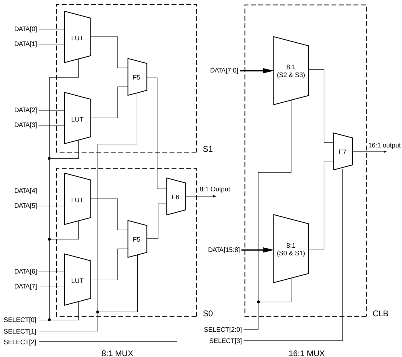
Figure 8-10: 8:1 and 16:1 Multiplexers
