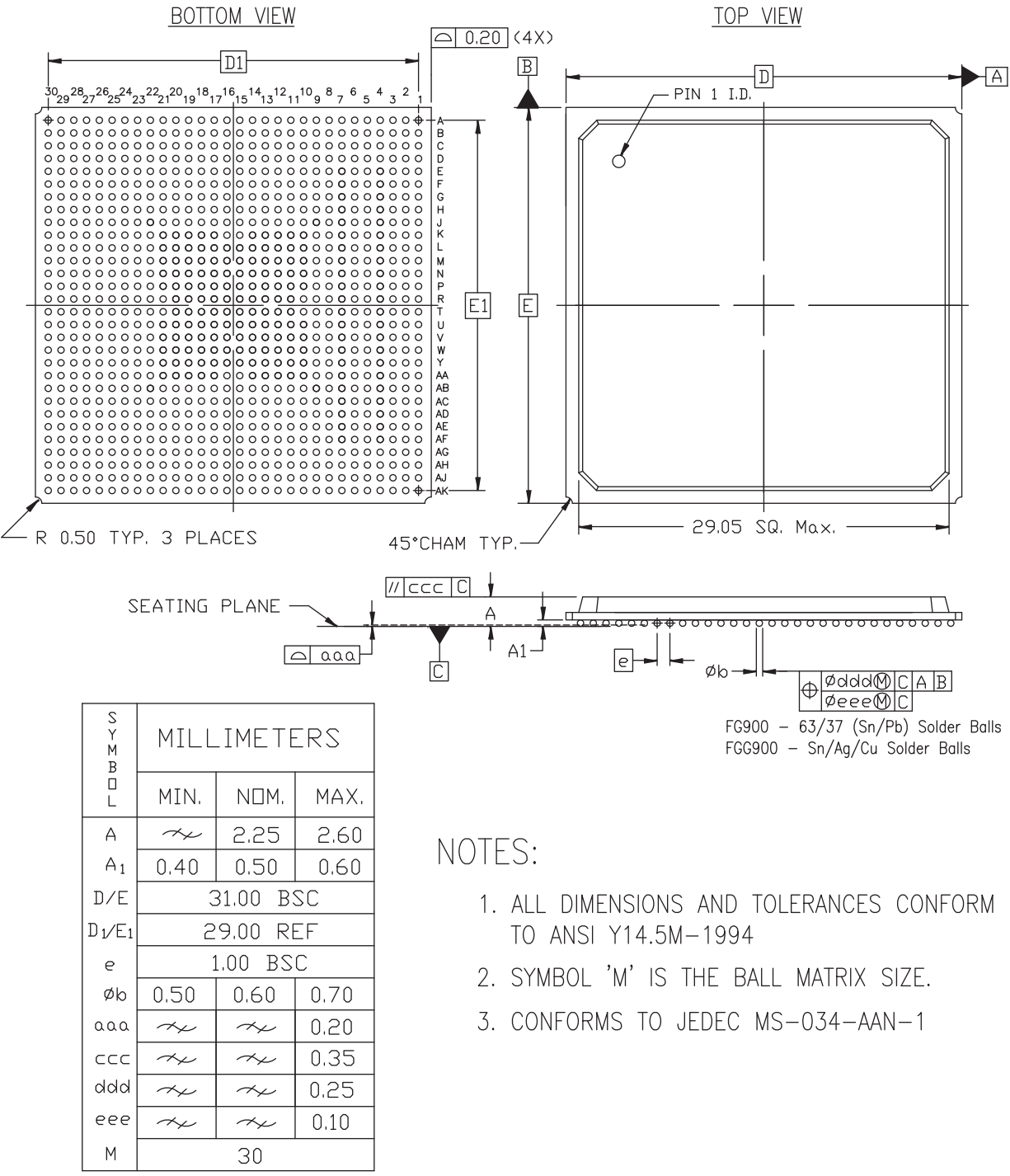
Figure 17-12: FG900/FGG900 Fine-Pitch BGA Package (pk038)
