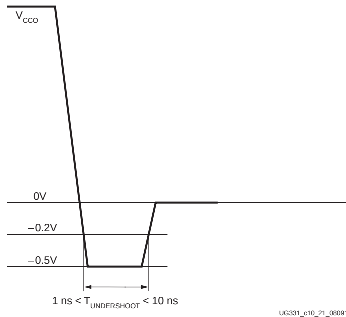
Figure 10-38: Timing Considerations for Input Undershoot
