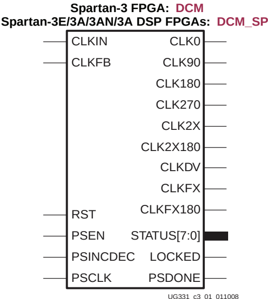
Figure 3-4: DCM Design Primitive
