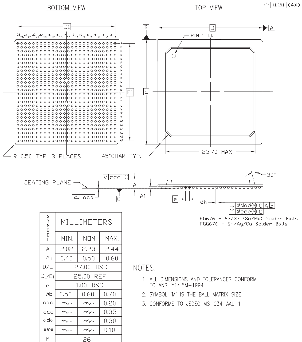
Figure 17-11: FG676/FGG676 Fine-Pitch BGA Package (pk035)
