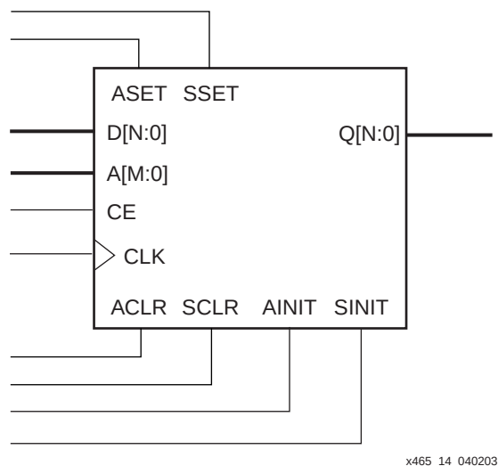
Figure 7-15: CORE Generator RAM-Based Shift Register Module
