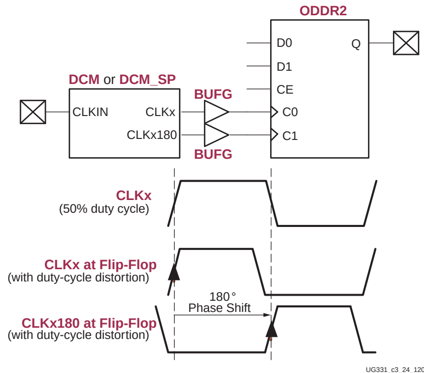
Figure 3-29: Using Half-Period Phase Shift Outputs Reduces Potential Duty-Cycle Distortion
