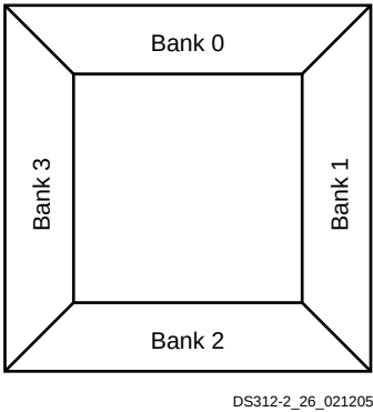
Figure 10-35: Spartan-3 Generation I/O Banks (top view)
