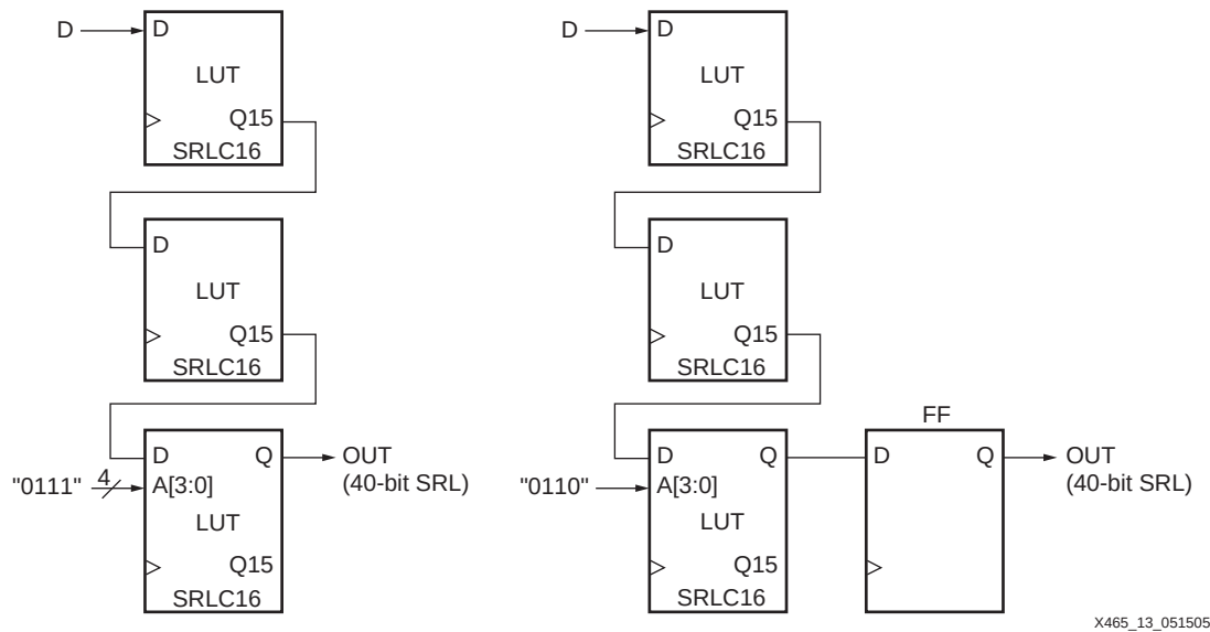
Figure 7-14: 40-bit Static-Length Shift Register
