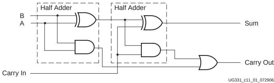
Figure 9-1: Full Adder
