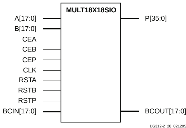
Figure 11-1: MULT18X18SIO Primitive
