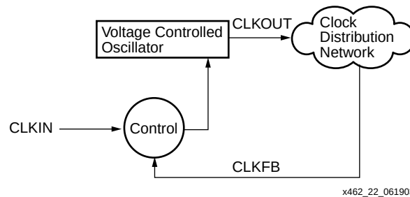
Figure 3-22: Phase-Locked Loop (PLL) Block Diagram
