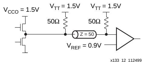
Figure 10-25: Terminated HSTL Class IV
