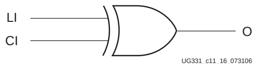
Figure 9-16: XORCY Primitive
