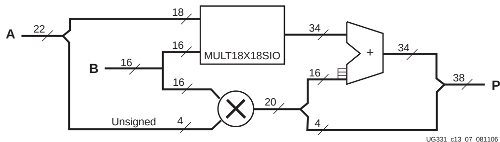
Figure 11-6: 22x16 Multiplier Implementation
