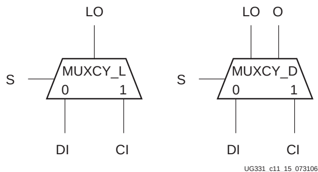
Figure 9-15: MUXCY_D and MUXCY_L Primitives
