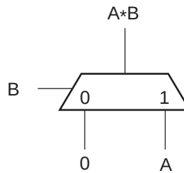
Figure 9-22: Using a MUXCY Multiplexer as an AND Gate
