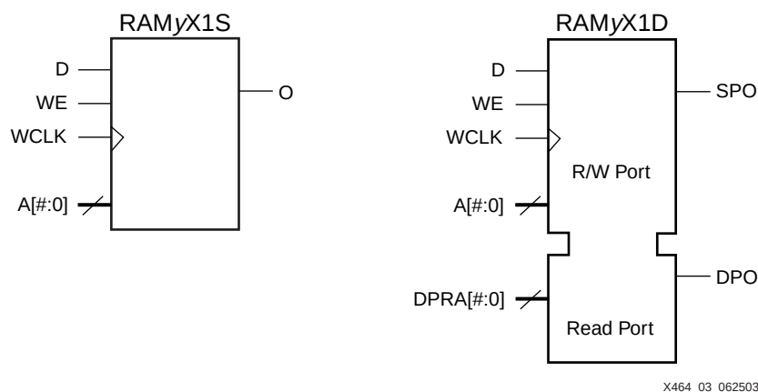
Figure 6-3: Single-Port and Dual-Port Distributed RAM Primitives
