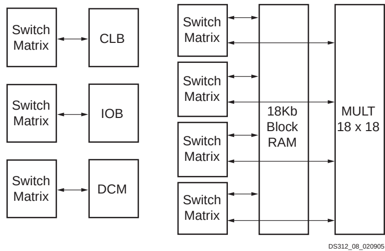
Figure 12-1: Four Types of Interconnect Tiles (CLBs, IOBs, DCMs, and Block RAM/Multiplier)
