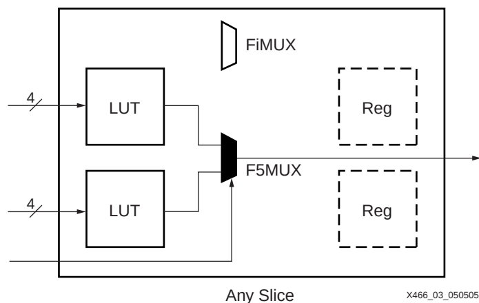
Figure 8-3: LUTs and F5MUX in a Slice
