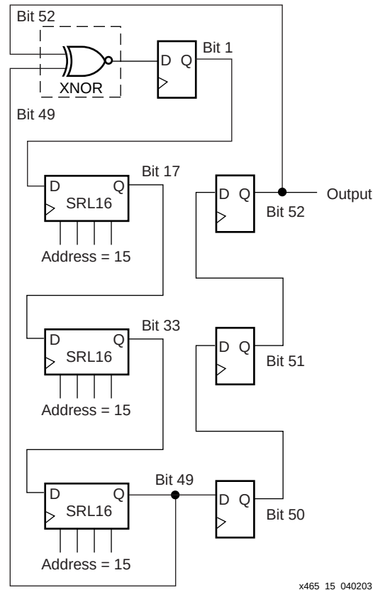
Figure 7-17: 52-bit LFSR
