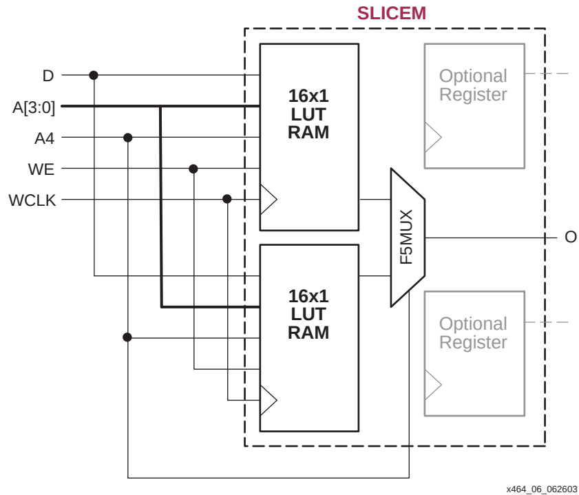
Figure 6-6: RAM32X1S Placement
