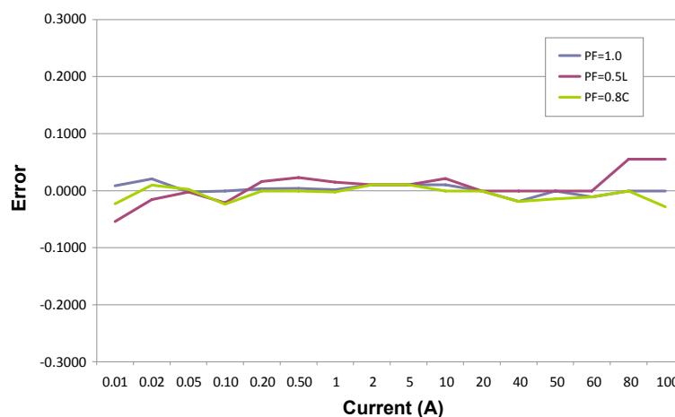
Figure 7. M90E36A Linearity
