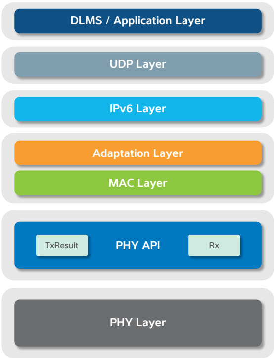
Figure 11. Atmel G3 Software Stack
