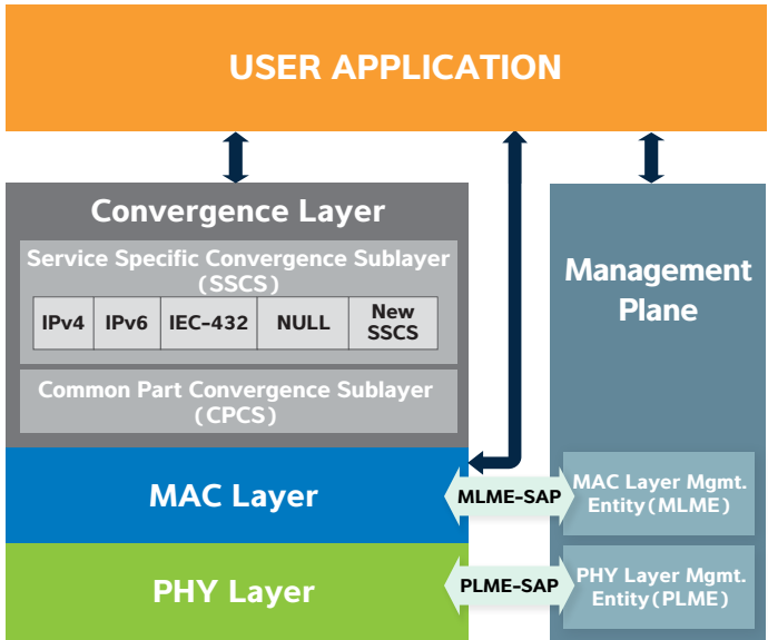
Figure 10. Atmel PRIME Software Stack
